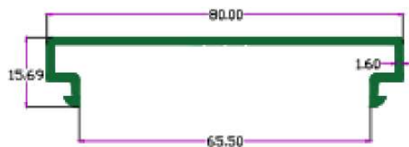
SEC. NO. 3875 Wt.1.90 TO 2.20 KG./ 12'
