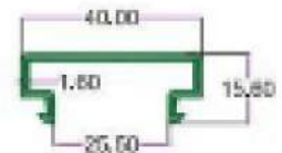
SEC. NO. 3877 WT. 1.200 TO 1.500 KG./ 12"
