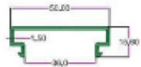
SEC. NO. 3873 WT. 1.300 TO 1.600 KG./ 12'
