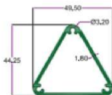
SEC. NO. 4122 WT. 2.850 TO 3.100 KG./12'
