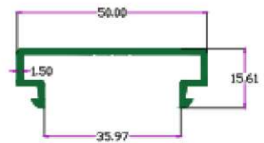
SEC. NO. 3873 Wt. 1.30 TO 1.600 KG./ 12'
