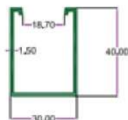
SEC. NO. 3869 WT. 1.400 TO 1.700 KG./ 12'
