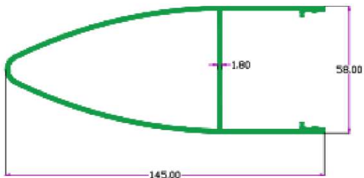
SEC. NO. 4700 Wt. 2.900 TO 3.120 KG./ 12'
