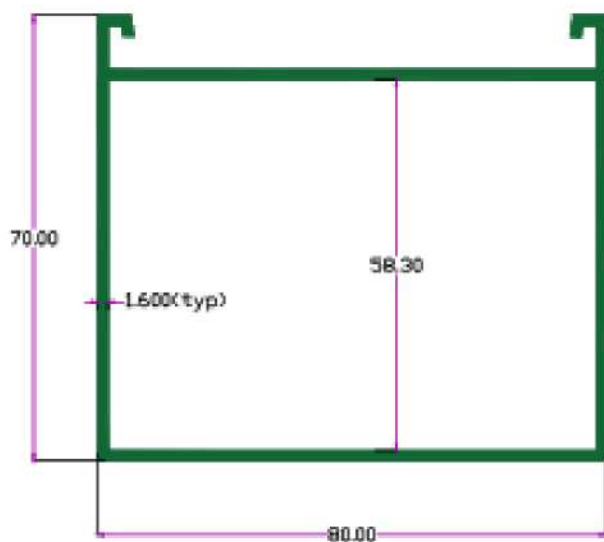
SEC. NO. 3874 Wt. 4.75 TO 5.100 KG./ 12'
