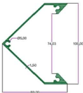
SEC. NO. 4121 WT. 4.800 TO 5.100 KG./12'
