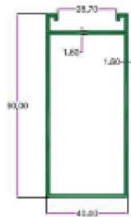
SEC. NO. 3876 WT. 4.100 TO 4.400 KG./ 12"
