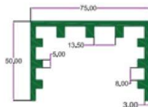
SEC. NO. 4134 WT. 7.350 TO 7.650 KG./12'
