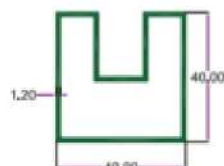
SEC. NO. 5128 WT. 2.310 TO 2.560 KG./12'
