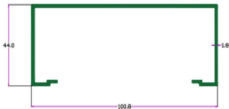
SEC. NO. 3251 Wt. 0.960 KG./ M
