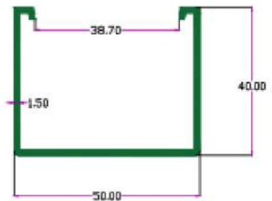
SEC. NO. 3872 Wt. 1.950 TO 2.300 KG./ 12'
