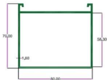
SEC. NO. 3874 WT. 4.75 TO 5.100 KG./ 12'
