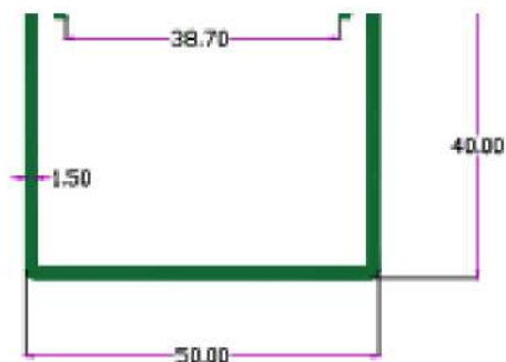
SEC. NO. 3872 Wt. 1.950 TO 2.300 KG./ 12'
