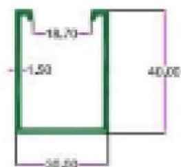
SEC. NO. 3869 WT. 1.400 TO 1.700 KG. / 12'
