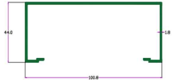
SEC. NO. 3251 Wt. 0.960 KG./ M
