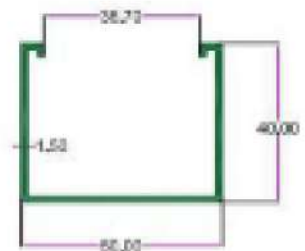
SEC. NO. 3872 WT. 1.950 TO 2.300 KG./ 12'
