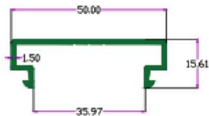
SEC. NO. 3873 Wt. 1.30 TO 1.600 KG./ 12'
