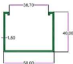
SEC. NO. 3872 WT. 1.950 TO 2.300 KG./ 12'
