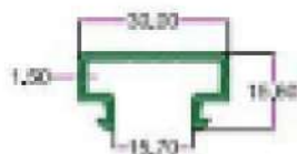
SEC. NO. 3870 WT. 1.200 TO 1.500 KG. / 12'
