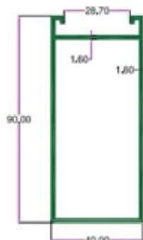
SEC. NO. 3876 WT. 4.100 TO 4.400 KG./ 12'
