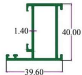
FRAME
