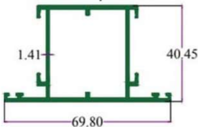
MULLION/Shutter
