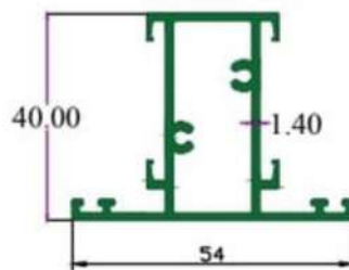
Mullion
