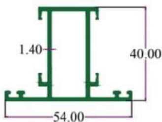
Shutter
