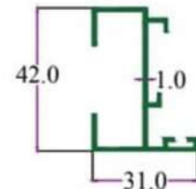
LAME-Z
