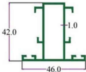
MULLION
