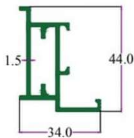
SEC. NO. 3261 WT. 2.026 TO 2.400 KG./ 12'
