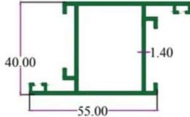
Z-MULLION
