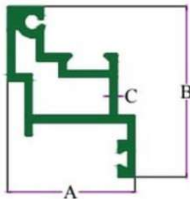
SEC. NO. 2180 WT. 1.900 TO 2.000 KG./ 12'
