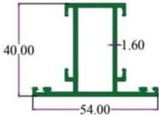
Shutter
