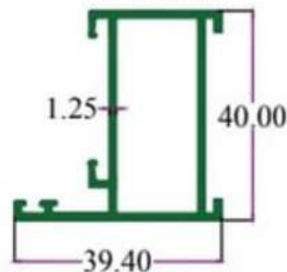
FRAME
