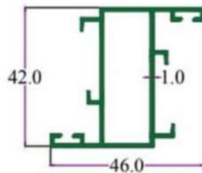
HOLLOW-Z
