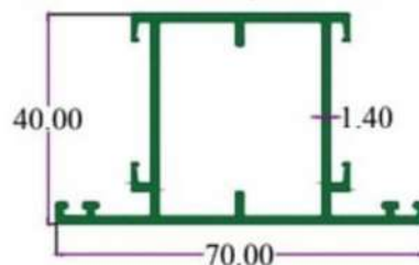
MULLION/Shutter
