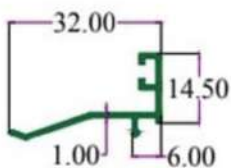
SEC. NO. 4773 WT. 0.600 TO 0.700 KG/12'
