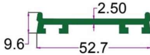
PRESSURE PLATE
