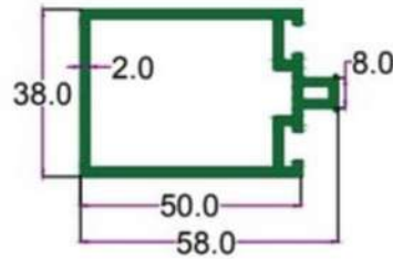
SEC. NO. 2509 WT. 3.000 TO 3.200 KG./12'
