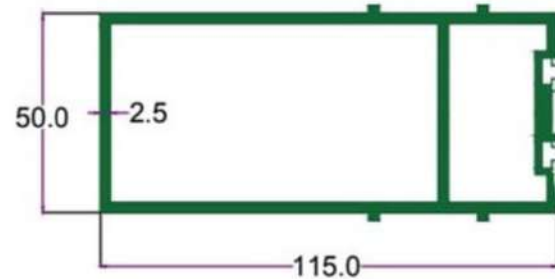
SEC. NO. 2512 WT. 9.370 TO 9.560 KG./12'
