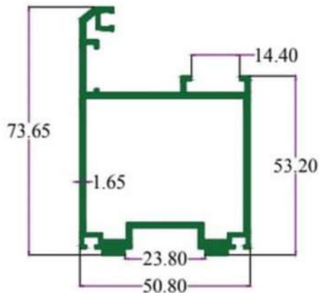
SEC. NO. 5006 WT. 4.735 TO 4.950 KG./ 12'
