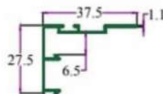
SEC. NO. 3312 WT. 0.940 TO 1.110 KG./12'
