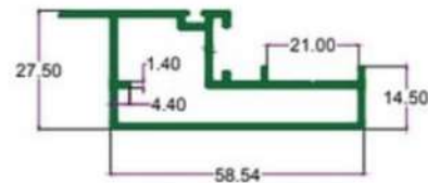
SEC. NO. 4142/D-6383 WT. 2.780 TO 3.00 KG./ 12'
