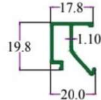
SEC. No. 3285 WT. 0.730 TO 0.850 KG./12'
