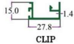
SEC. NO. 2164 WT. 1.050 TO 1.240 K./15'
