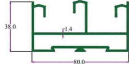
SEC. NO. 3314 WT. 4.30 TO 4.50 KG./ 12'
