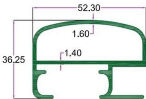
SEC.NO. 4336 WT. 3.200 TO 3.450 KG/12'
