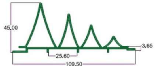
SEC. NO. 4549 WT. 4.800 TO 5.000 KG./ 12'
