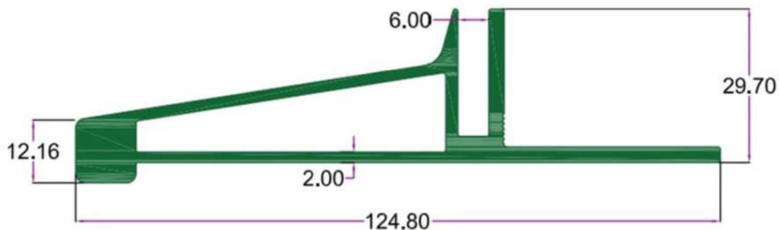
SEC. NO. 4335 WT. 6.960 TO 7.200 KG/12'
