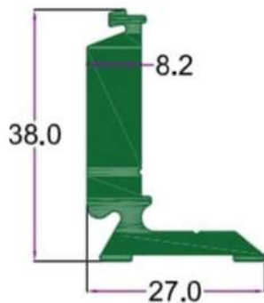
SEC. NO. 3666 WT. 3.200 TO 3.500 KG/I2'
