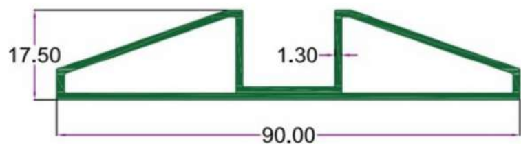
SEC. NO. 5143 WT. 2.820 TO 3.070 KG/12'
