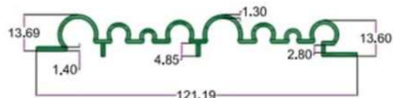
SEC. NO. 4541 WT. 3.080 TO 3.250 KG./12'
