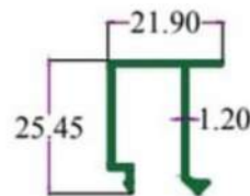
SEC. NO. 5007 WT. 0.940 TO 1.100 KG./ 12'
