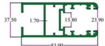
SEC. NO. 4748 WT. 5.240 TO 5.500 KG. / 12'
