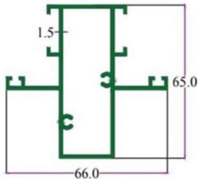
SEC. NO. 3531 WT. 3.800 TO 4.200 KG / 12'
