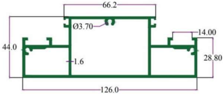
SEC. NO. 3527 WT. 7.100 TO 7.900 KG / 12'
