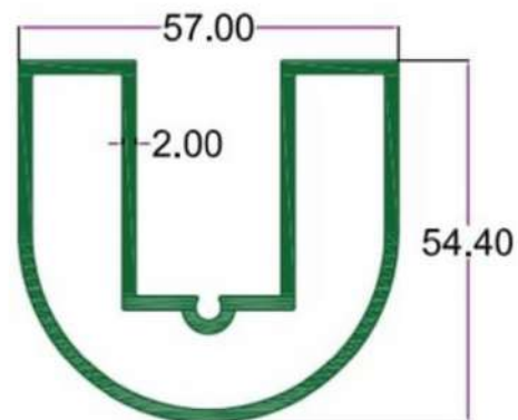
SEC.NO. 5178 WT. 5.270 TO 5.520 KG/12'
