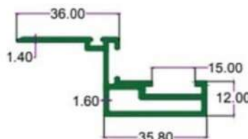
SEC. NO. 4140/D-4629 WT. 2.370 TO 2.560 KG./ 12'
