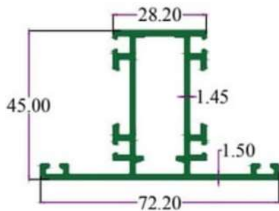
SEC.NO. 4930 WT. 3.720 TO 3.980 KG./ 12'
