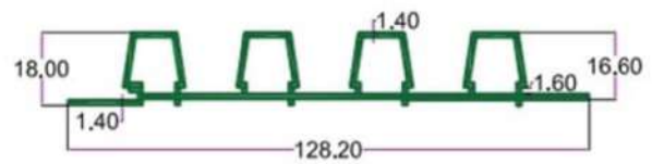
SEC. NO. 4126 WT. 4.150 TO 4.300 KG./12'
