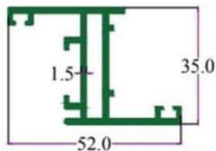
SEC. NO. 3517 WT. 2.300 TO 2.600 KG / 12'
