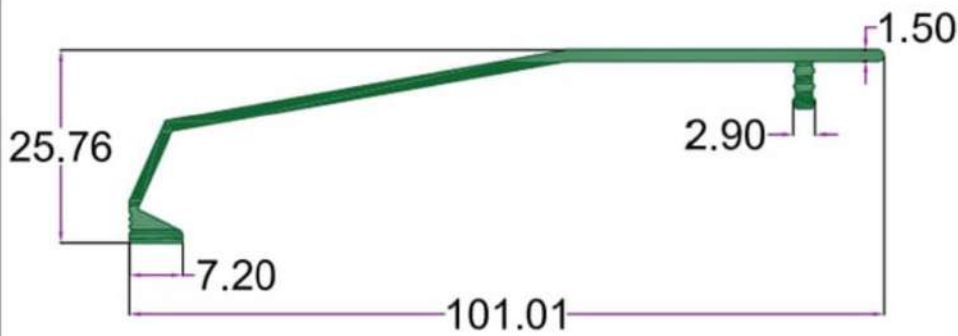
SEC. NO. 4273 WT. 1.950 TO 6.280 KG/I2'
