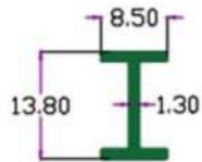
SEC.NO. 4764 Wt. 0.360 TO 0.460 KG./ 12'
