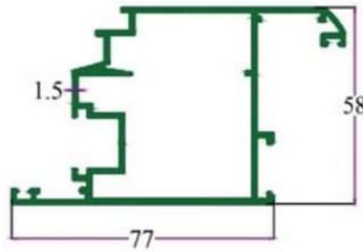
SEC.NO. 4774 WT. 5.150 TO 5.400 KG/12'
