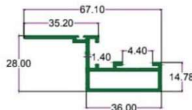
SEC. NO. 2456 WT. 2.340 TO 2.550 KG/15'
