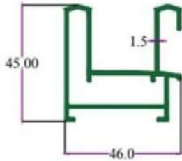
SEC. NO. 3313 WT. 3.270 TO 3.550 KG./ 12'
