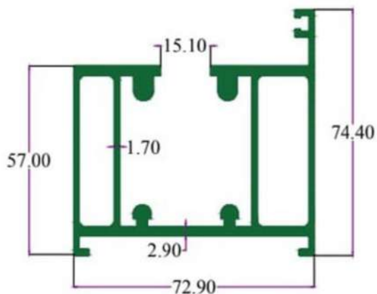
SEC. NO. 5008 WT. 8.860 TO 9.000 KG./ 12'
