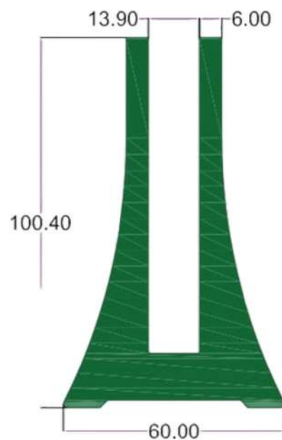
SEC.NO. 5198 WT. 21.450 TO 21.950 KG/12'
