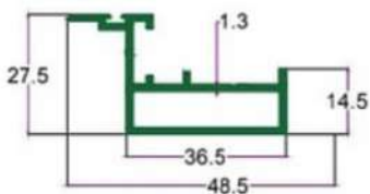
SEC. NO. 2448 WT. 2.370 TO 2.550 KG/ 15'
