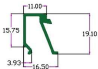
SEC. NO. 3773 Wt. 0.60 TO 0.80 KG / 12'
