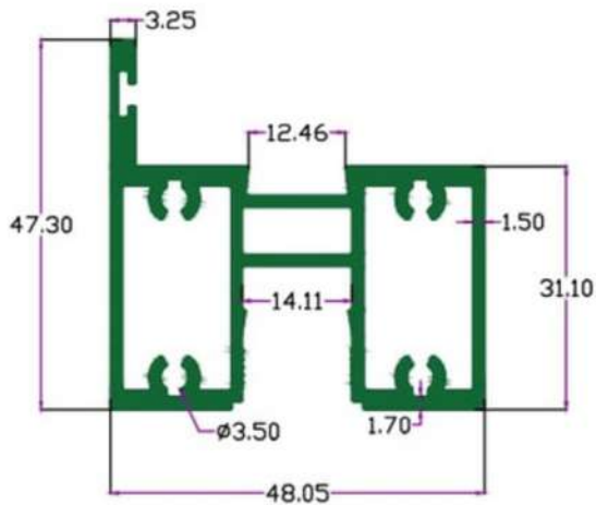
SEC.NO. 4764 Wt. 0.360 TO 0.460 KG./ 12'
