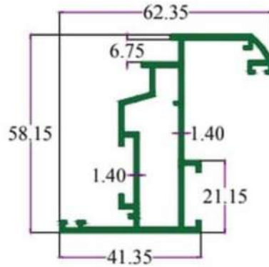
SEC. NO. 4768 WT. 3.320 TO 3.520 KG/12'
