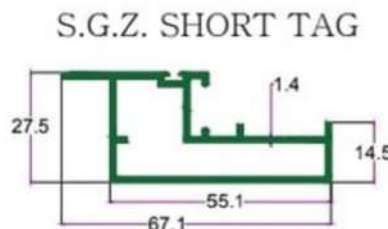
SEC. NO. 2450 (L) WT. 3.230 TO 3.400 KG/15' (H) WT. 4.120 TO 4.250 KG/15'
