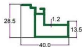
SEC. NO. 3201 WT. 1.680 TO 1.900 KG/15'
