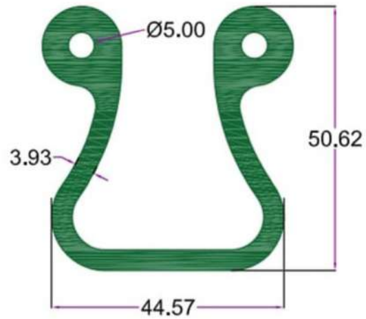
SEC.NO. 4702 WT. 7.570 TO 7.820 KG/12'
