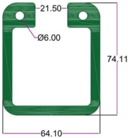
SEC.NO. 4399 WT. 15.600 TO 16.150 KG/12'
