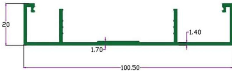
SEC. NO. 3897 Wt. 2.500 TO 2.800 KG. / 12'
