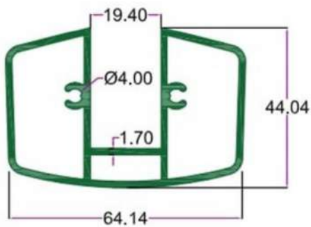
SEC.NO. 4642 WT. 4.940 TO 5.200 KG/12'
