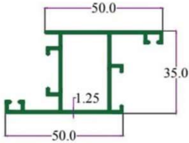
SEC. No. 3284 WT. 2.540 TO 2.800 KG./ 12'
