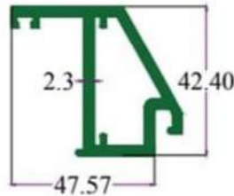
SEC. NO. 2182 WT. 3.950 TO 4.100 KG/15'
