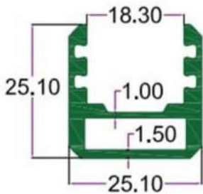
SEC. NO. 3539 WT. 1.800 TO 2.100 KG/12'
