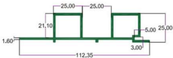
SEC. NO. 4801 WT. 4.000 TO 4.250 KG./ 12'
