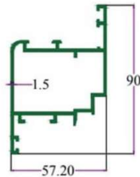
SEC. NO. 3940 WT. 4.400 TO 4.80 KG/12'
