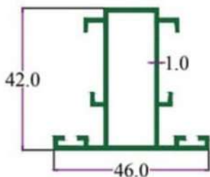
SEC. NO. 2161 WT. 2.200 TO 2.700 KG/15'
