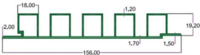
SEC. NO. 4512 WT. 6.050 TO 6.250 KG./ 12'
