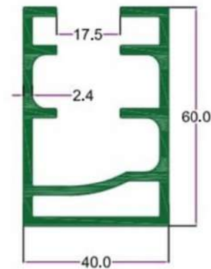
SEC. NO. 3535 WT. 5.600 TO 6.300 KG/12'
