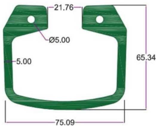
SEC.NO. 4641 WT. 15.250 TO 15.500 KG/12'
