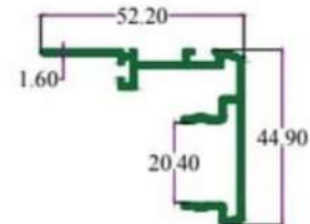
SEC. NO. 4710 WT. 2.420 TO 2.610 KG. / 12'
