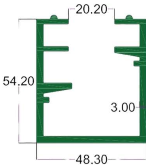
SEC.NO. 5110 WT. 6.165 TO 6.415 KG/12'
