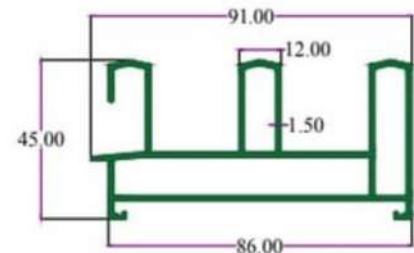
SEC. NO. 4272 WT. 5.750 TO 6.100 KG./ 12'
