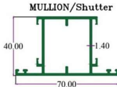
SEC. NO. 3484 WT. 3.950 TO 3.250 KG/12'
