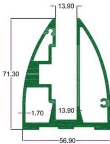
SEC. NO. 4395 WT. 8.300 TO 8.650 KG/12'
