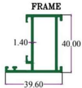
SEC. NO. 3482 WT. 2.100 TO 2.400 KG/12'
