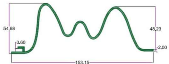
SEC. NO. 4532 WT. 5.670 TO 5.850 KG./ 12'
