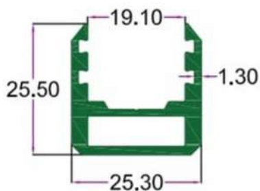
SEC. NO. 4408 WT. 1.900 TO 2.100 KG/12'
