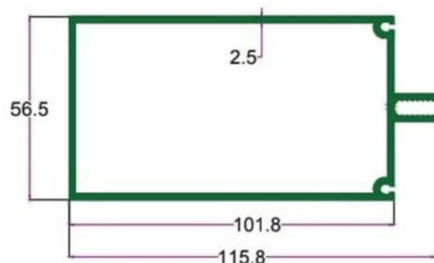
SEC. NO. 2437 WT. 10.850 TO 11.220 KG./15'
