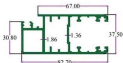
SEC. NO. 4711 WT. 4.820 TO 5.050 KG. / 12'
