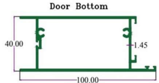
SEC. NO. 3485 WT. 4.100 TO 4.600 KG/12'
