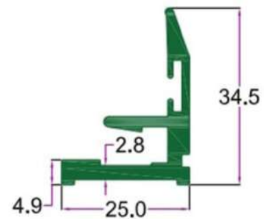
SEC. NO. 2885 WT. 2.000 TO 2.300 KG/I2'
