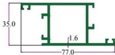
SEC. NO. 3520 WT. 3.100 TO 3.500 KG / 12'
