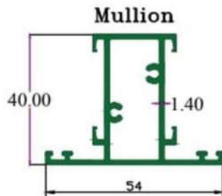
SEC. NO. 3481 WT. 2.600 TO 2.900 KG/12'
