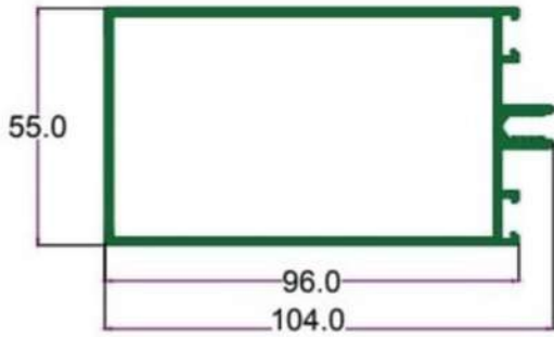
SEC. NO. 2430 (L) WT. 5.680 TO 5.850 KG/12' (H) WT. 6.640 TO 6.850 KG/12'
