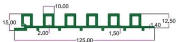
SEC. NO. 4378 WT. 5.780 TO 6.000 KG./12'
