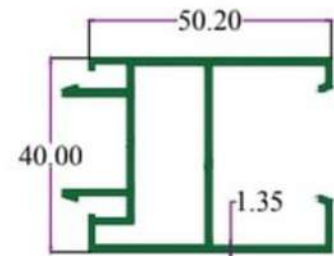
SEC. NO. 3783 WT. 2.850 TO 3.00 KG/12'
