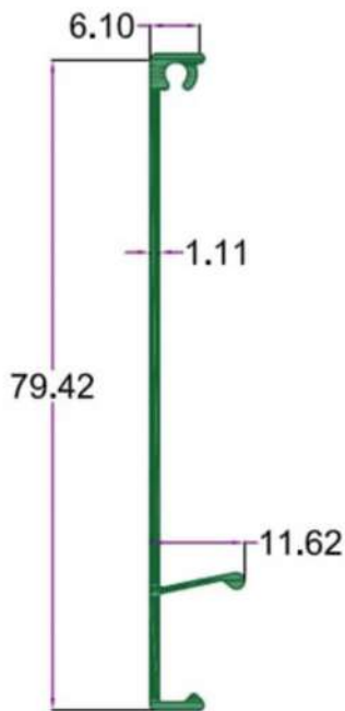
SEC.NO. 4668 WT. 1.150 TO 1.300 KG/12'
