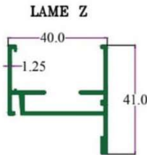
SEC. NO. 2054 WT. 2.900 TO 3.100 KG./ 15'
