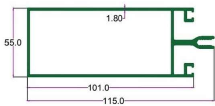
SEC. NO. 2431 WT. 8.400 TO 8.600 KG/12'
