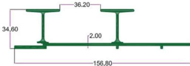
SEC. NO. 4098 WT. 5.900 TO 6.200 KG./ 12'
