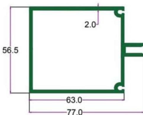
SEC. NO. 2436 WT. 7.000 TO 7.500 KG/15'
