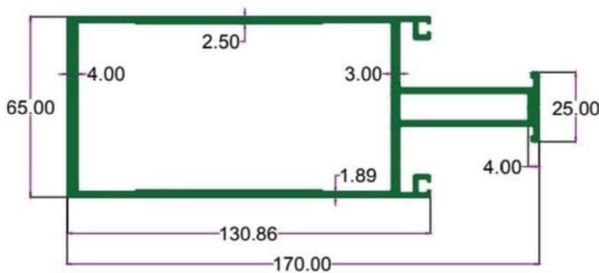
SEC. NO. 4592 WT. 12.950 TO 13.350 KG./ 12'
