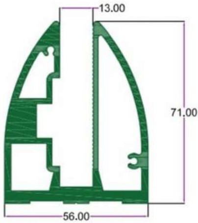
SEC. NO. 3497 WT. 10.700 TO 11.200 KG/12'
