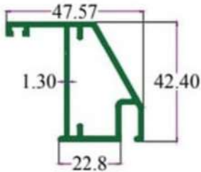
SEC. NO. 2181 WT. 1.900 TO 2.200 KG/12'
