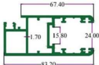
SEC. NO. 4747 WT. 5.700 TO 5.950 KG. / 12'
