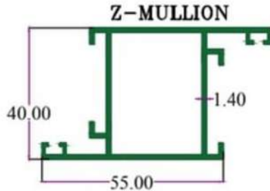
SEC.NO. 3339 WT. 3.050 To 3.250 KG/12'
