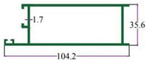
SEC. NO. 2064 WT. 4.647 TO 8.000 KG. / 12'
