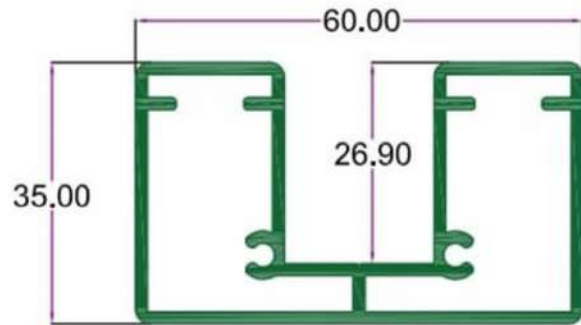
SEC. NO. 3925 WT. 4.200 TO 4.500 KG/12'
