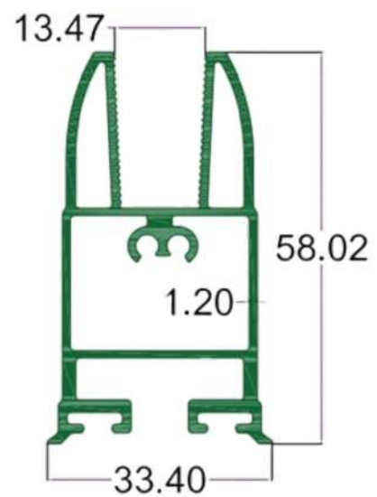
SEC.NO. 5111 WT. 3.648 TO 3.895 KG/12'
