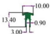
SEC.NO. 4846 WT. 0.470 TO 0.570 KG./ 12'
