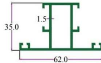
SEC. NO. 3515 WT. 2.300 TO 2.600 KG / 12'
