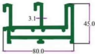
SEC. NO. 3694 WT. 9.60 TO 10.60 KG / 12'
