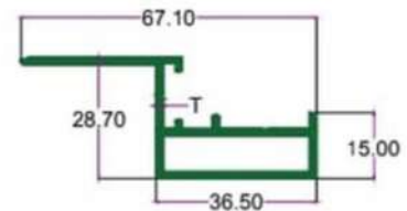
SEC. NO. 2457 WT. 1.960 TO 2.250 KG/15'
