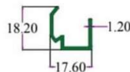
SEC. NO. 3995 WT. 0.500 TO 0.700 KG./12'
