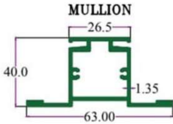
SEC. NO. 2051 WT. 3.900 TO 4.200 KG/15'
