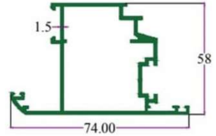
SEC.NO. 4775 WT. 3.320 TO 3.520 KG/12'
