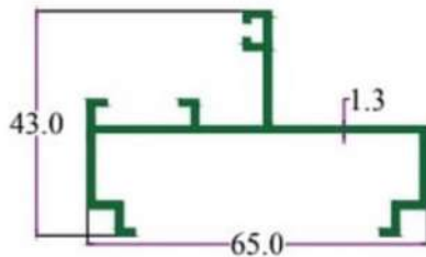
SEC. NO. 3528 WT. 2.050 TO 2.300 KG / 12'
