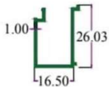
SEC. NO. 3781 WT. 0.70 TO 0.90 KG/12'
