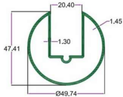
SEC. NO. 4349 WT. 2.820 TO 3.000 KG/12'
