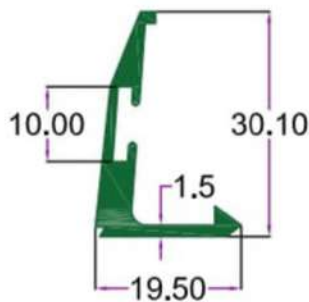
SEC. NO. 2884 WT. 1.100 TO 1.350 KG/I2'
