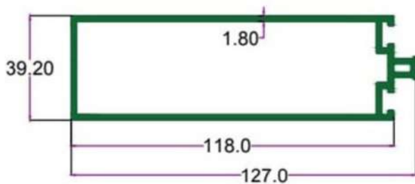
SEC. NO. 2508 WT. 6.530 TO 6.750 KG./12'
