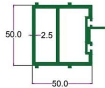
SEC. NO. 2510 WT. 6.260 TO 6.400 KG./12'
