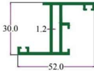
SEC. NO. 3523 WT. 1.650 TO 1.850 KG / 12'
