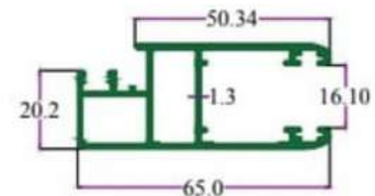
SEC. NO. 3331 WT. 3.100 TO 3.400 KG./ 12'
