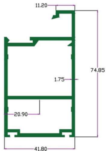
SEC. NO. 3772 Wt. 4.80 TO 5.10 KG / 12'
