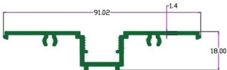
SEC. NO. 3898 Wt. 2.400 TO 1.700 KG. / 12'
