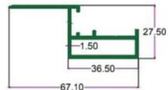
SEC. NO. 2460 WT. 2.700 TO 2.900 KG./ 15'
