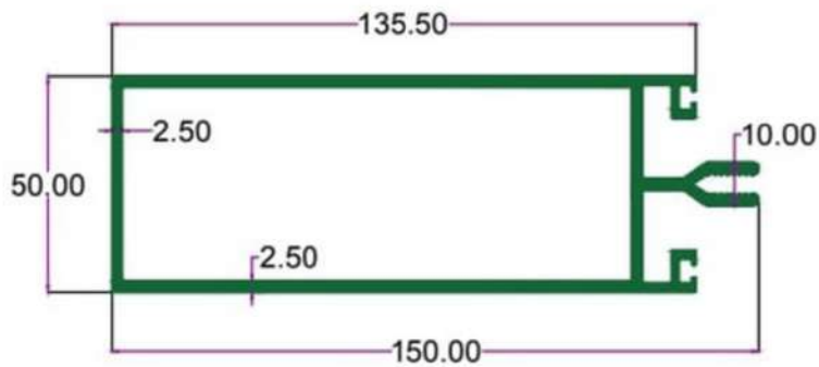
SEC. NO. 4160 WT. 10.400 TO 10.900 KG/12'
