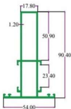
SEC. NO. 4271 WT. 3.500 TO 3.800 KG./ 12'
