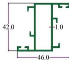
SEC. NO. 2162 WT. 2.300 TO 2.800 KG/15'
