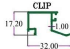
SEC.NO. 3341N WT. 0.750 To 0.850 KG/12'
