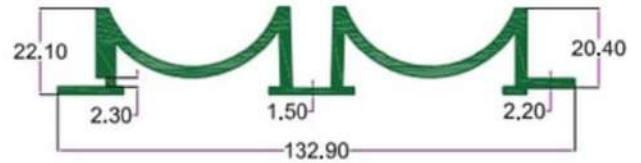
SEC. NO. 4096 WT. 6.450 TO 6.750 KG./12'
