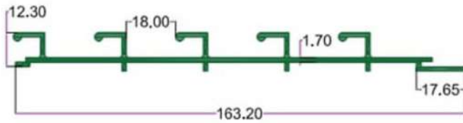
SEC. NO. 4130 WT. 4.600 TO 4.850 KG./12'
