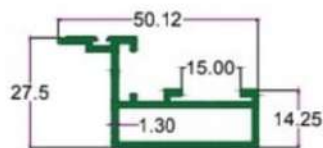
SEC. NO. 2448A (L) WT. 2.820 TO 3.000 KG/15' (H) WT. 3.120 TO 3.250 KG/15'
