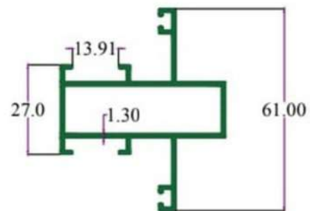
SEC. NO. 3521 WT. 3.000 TO 3.300 KG / 12'
