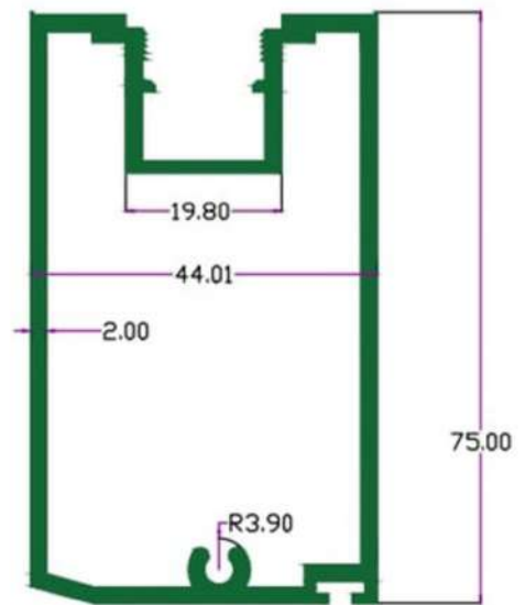
SEC. NO. 3777 Wt. 5.50 TO 5.80 KG / 12'
