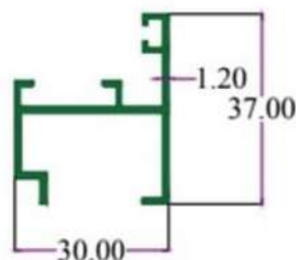
SEC. NO. 3994 WT. 1.300 TO 1.600 KG./12'
