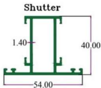
SEC. NO. 3483 WT. 2.350 TO 2.650 KG/12'
