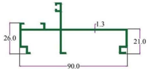
SEC. NO. 3529 WT. 2.700 TO 3.000 KG / 12'
