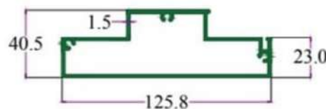
SEC. NO. 2063 WT. 5.260 TO 5.450 KG/12'
