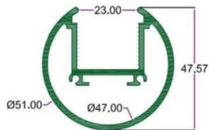
SEC. NO. 3498 WT. 4.180 TO 4.580 KG/12'
