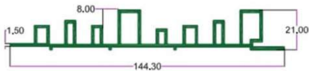
SEC. NO. 4872 WT. 5.820 TO 6.100 KG./ 12'
