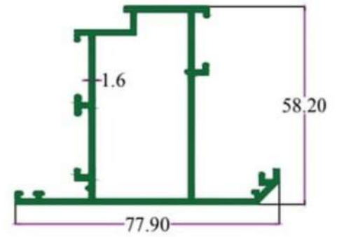
SEC. NO. 3780 WT. 4.200 TO 4.500 KG/12'
