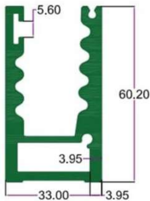
SEC.NO. 5112 WT. 7.080 TO 7.335 KG/12'
