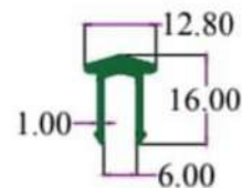
SEC.NO. 4890 WT. 0.555 TO 0.660 KG./ 12'
