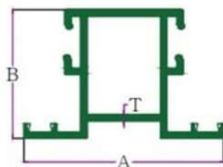
MULLION SECTION
