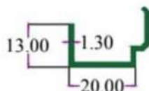
SEC. NO. 3526 WT. 0.630 TO 0.710 KG/12'
