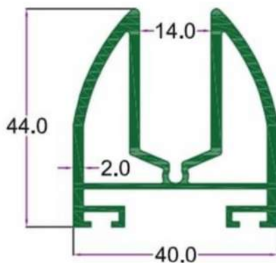
SEC. NO. 3536 WT. 3.650 TO 4.100 KG/12'
