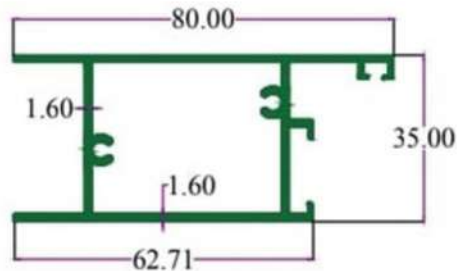
SEC. NO. 3519 WT. 3.600 TO 4.000 KG / 12'
