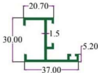
SEC. NO. 3522 WT. 1.550 TO 1.750 KG / 12'
