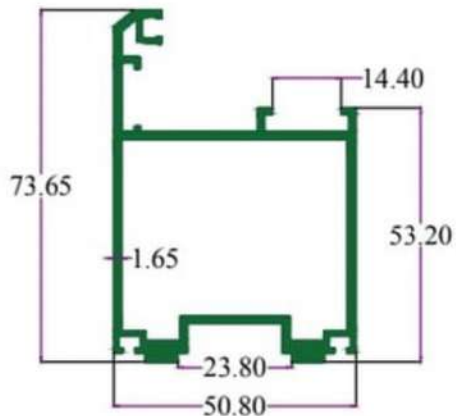
SEC. NO. 5006 WT. 4.735 TO 4.950 KG./ 12'
