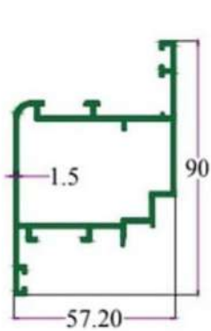
SEC. NO. 3940 WT. 4.400 TO 4.80 KG/12'
