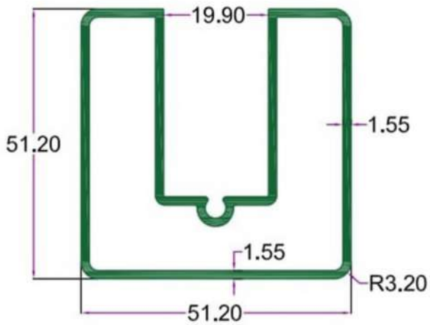
SEC.NO. 4369 WT. 4.120 TO 4.300 KG/12'
