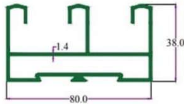
SEC. NO. 3316 WT. 4.290 TO 4.500 KG./ 12'
