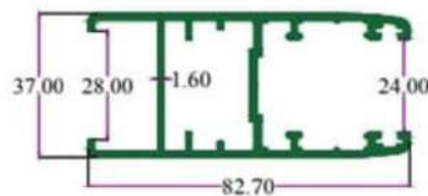
SEC. NO. 4709 WT. 4.610 TO 4.850 KG. / 12'
