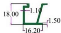
SEC.NO. 4893 WT. 0.580 TO 0.680 KG./ 12'
