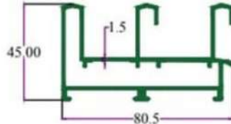
SEC. NO. 3311 WT. 5.200 TO 5.400 KG./ 12'
