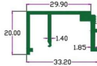
SEC. NO. 3775 Wt. 1.35 TO 1.50 KG / 12'
