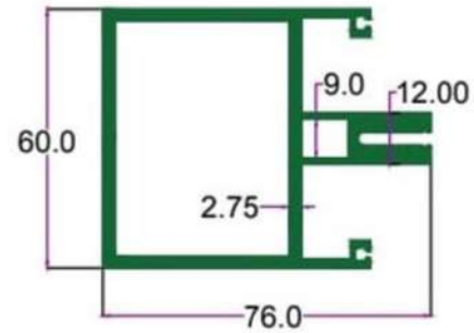
SEC. No. 2439 WT. 8.000 TO 8.500 KG./12'
