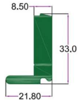
SEC. NO. 3665 WT. 3.075 TO 3.350 KG/I2'
