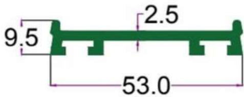
PRESSURE PLATE
