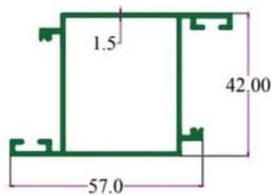
SEC. NO. 2204 WT. 2.600 TO 3.100 KG/15'
