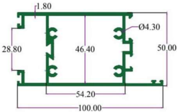
SEC. NO. 4769 WT. 6.550 TO 6.800 KG/12'
