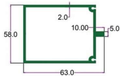
SEC. NO. 2434 WT. 6.500 TO 7.200 KG/15'
