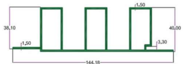
SEC. NO. 4542 WT. 6.390 TO 6.550 KG./ 12'
