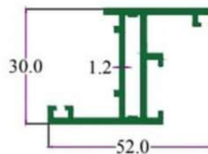
SEC. NO. 3525 WT. 1.650 TO 1.850 KG / 12'
