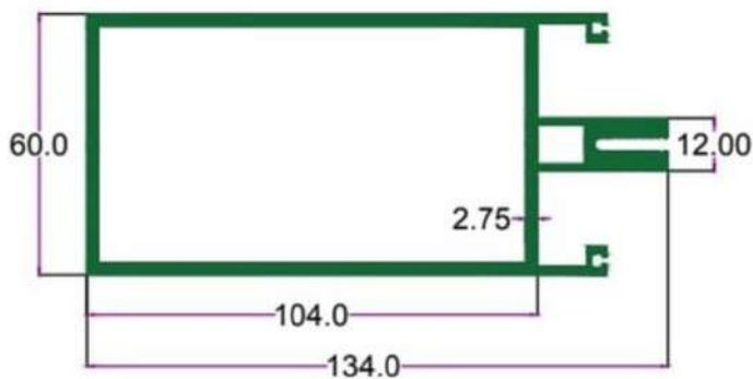
SEC. No. 2438 WT. 12.390 TO 12.600 KG/12'
