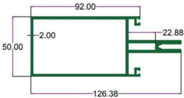
SEC. NO. 2461 WT.7.450 To 7.750 KG./15'
