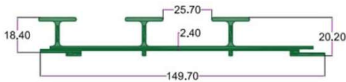
SEC. NO. 4094 WT. 5.900 TO 6.300 KG./ 12'
