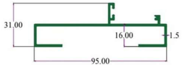
SEC. NO. 2202 WT. 2.600 TO 3.100 KG/15'
