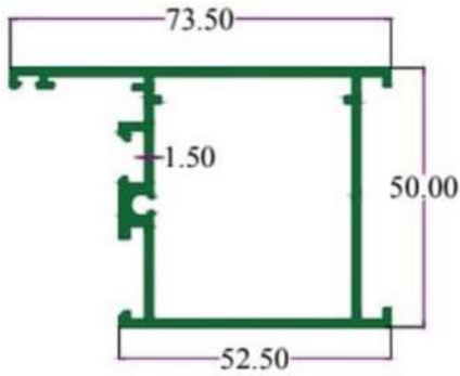
SEC.NO. 4771 WT. 3.320 TO 3.520 KG/12'
