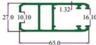
SEC. NO. 3315 WT. 2.720 TO 3.000 KG./12'
