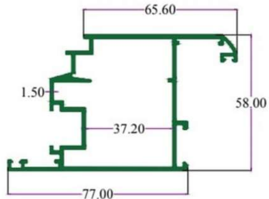
SEC. NO. 4774 WT. 5.150 TO 5.400 KG/12'
