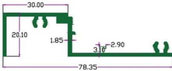
SEC. NO. 3774 Wt. 2.25 TO 2.50 KG / 12'
