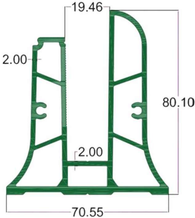
SEC.NO. 5179 WT. 9.560 TO 9.810 KG/12'
