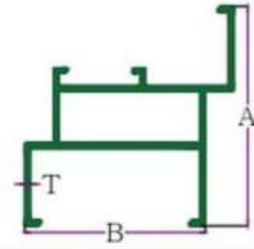
Z BOX SECTION
