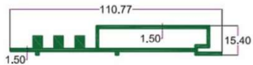
SEC. NO. 4479 WT. 4.040 TO 4.250 KG/ 12'
