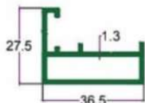
SEC. NO. 2449 , (L) WT. 1.990 TO 2.100 KG/15' (H) WT. 3.120 TO 3.300 KG/15'
