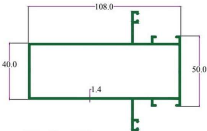
SEC. No. 3287 WT. 5.240 TO 5.500 KG./ 12'
