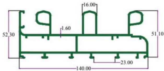
SEC. NO. 4713 WT. 9.810 TO 10.120 KG. / 12'
