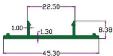
SEC.NO. 4692 Wt. 0.740 TO 0.850 KG./ 12'
