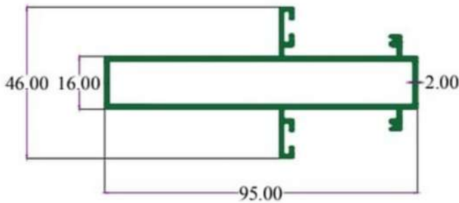
SEC. NO. 2201 WT. 3.900 TO 4.400 KG/15'
