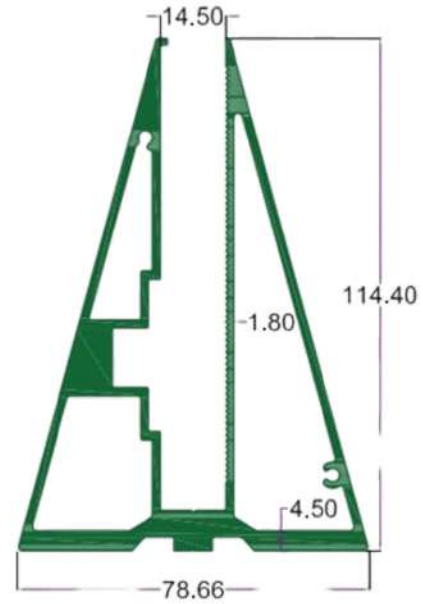
SEC.NO. 4606 WT. 12.870 TO 13.100 KG/12'
