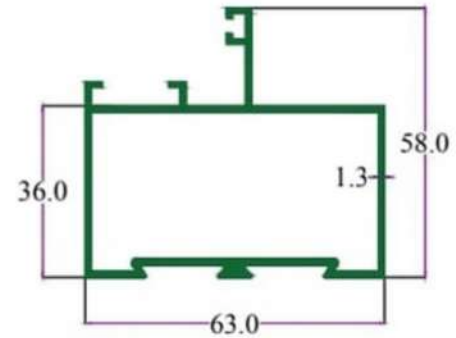
SEC. NO. 3530 WT. 3.100 TO 3.500 KG / 12'
