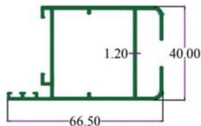
SEC. NO. 3464 WT. 3.500 TO 3.700 KG./ 12'
