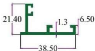
SEC. NO. 2065 WT. 1.000 TO 1.200 KG. / 12'
