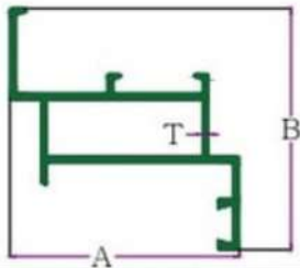
Z HOLLOW SECTION
