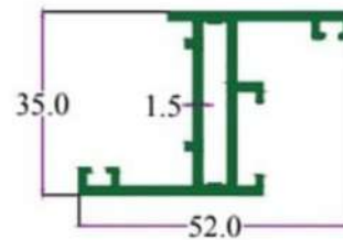
SEC. NO. 3516 WT. 2.200 TO 2.500 KG / 12'
