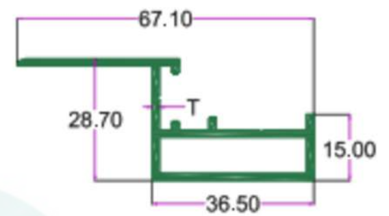
SEC. NO. 2457 WT. 1.960 TO 2.250 KG/15'
