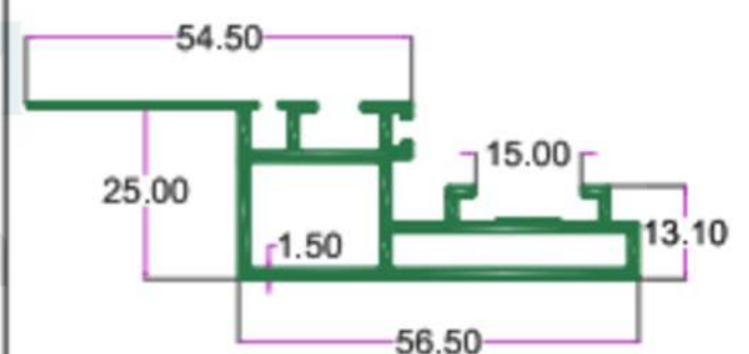
SEC. NO. 4593 WT. 3.280 TO 3.450 KG/12'
