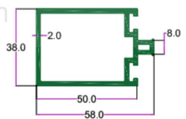
SEC. NO. 2509 WT. 3.000 TO 3.200 KG/12'
