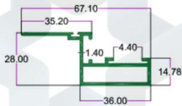
SEC. NO. 2456 WT. 2.340 TO 2.550 KG/15'
