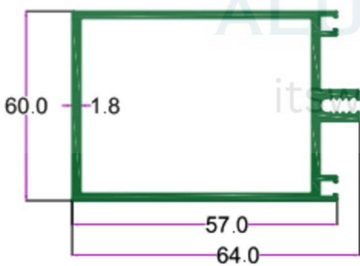
SEC. NO. 2435 WT. 6.800 TO 7.300 KG./15'
