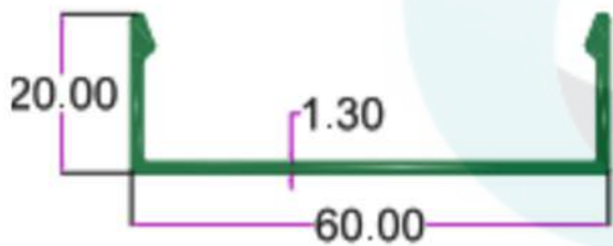
SEC. NO. 4114 WT. 1.300 TO 1.450 KG/12'
