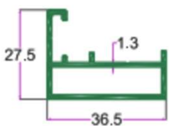
SEC. NO. 2449 (L) WT. 1.990 TO 2.100 KG/15' (H) WT. 3.120 TO 3.300 KG/15'
