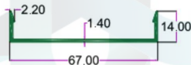
SEC.NO. 5314 WT. 0.250 TO 0.500 KG/12'
