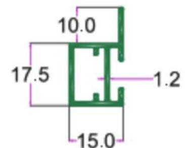
SEC. NO. 2503 WT. 0.900 TO 1.100 KG/I2'
