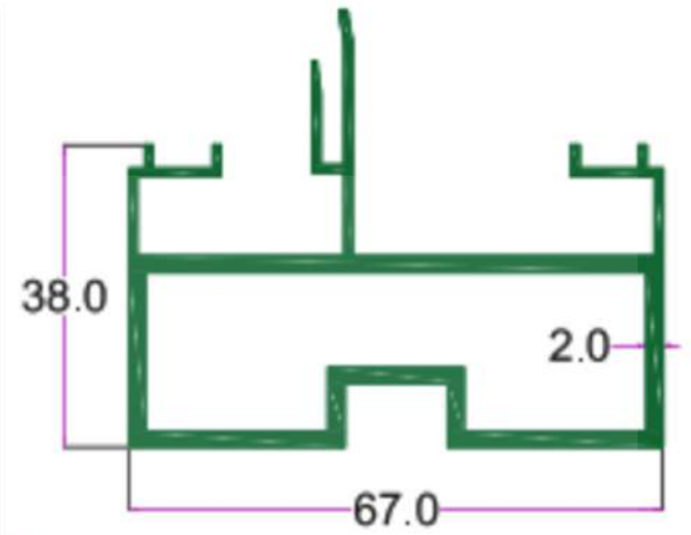
SEC. NO. 245I WT. 5.300 TO 5.800 KG/I5'
