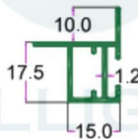
SEC. NO. 2502 WT. 1.060 TO 1.200 KG/I2'
