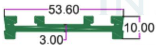
SEC.NO. 5218 WT. 2.375 TO 2.625 KG/12'
