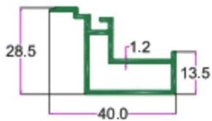
SEC. NO. 3201 WT. 1.680 TO 1.900 KG/15'
