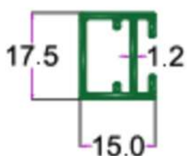
SEC. NO. 2504 WT. 0.830 TO 1.000 KG/I2'
