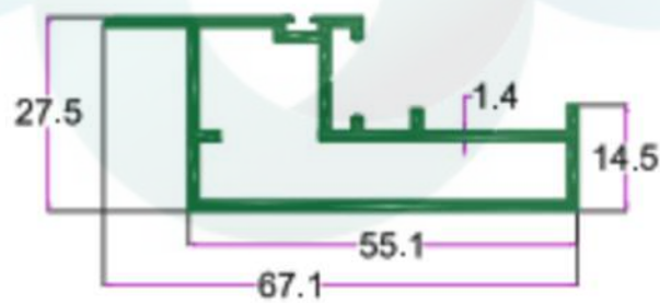
SEC. NO. 2450 (L) WT. 3.230 TO 3.400 KG/15' (H) WT. 4.120 TO 4.250 KG/15'
