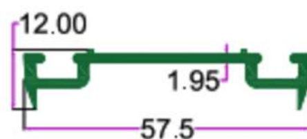
SEC. No. 2440 WT. 1.400 TO 1.600 KG/12'
