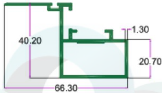
SEC. NO. 4196 WT. 2.450 TO 2.650 KG/12'
