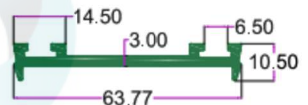
SEC.NO. 5315 WT. 2.360 TO 2.610 KG/12'
