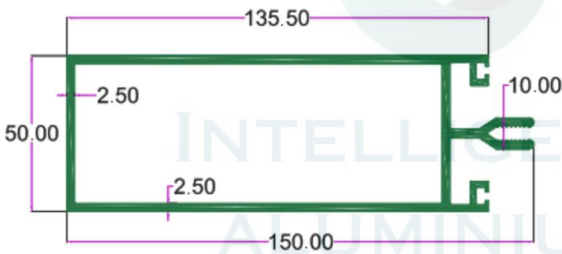
SEC. NO. 4160 WT. 10.400 TO 10.900 KG/12'
