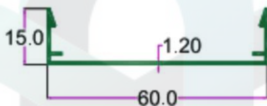
SEC. No. 2441 WT. 0.800 TO 0.900 KG/12'
