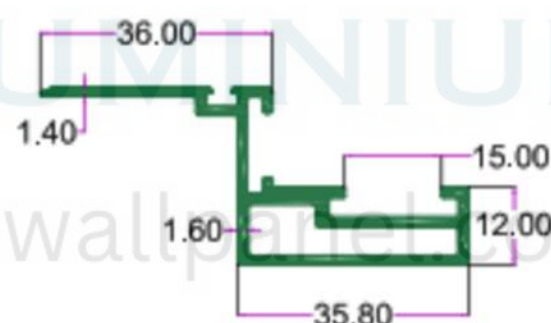
SEC. NO. 4140/D-4629 WT. 2.370 TO 2.560 KG/12'
