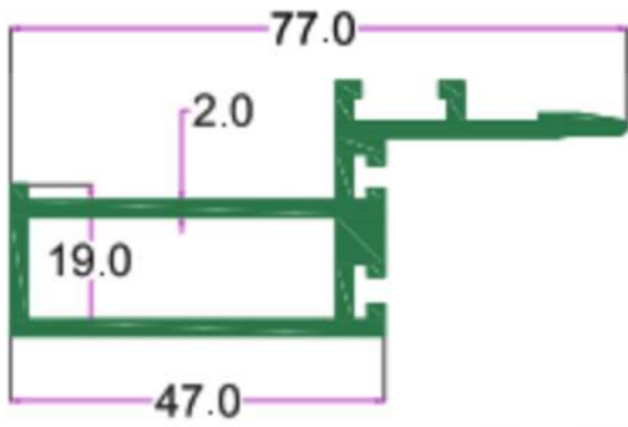
SEC. NO. 2453 WT. 3.900 TO 4.400 KG/I5'
