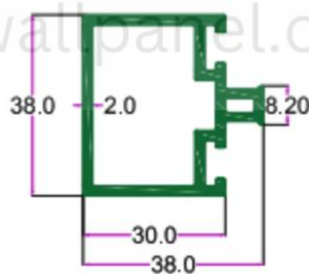
SEC. NO. 2505 WT. 3.080 TO 3.250 KG/12'
