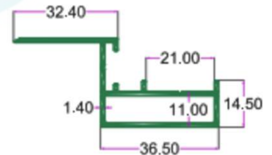
SEC. NO. 4141/D-6859 WT. 2.040 TO 2.200 KG/12'
