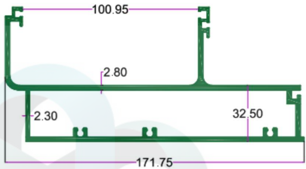
SEC.NO. 4986 WT. 14.050 TO 14.600 KG/12'
