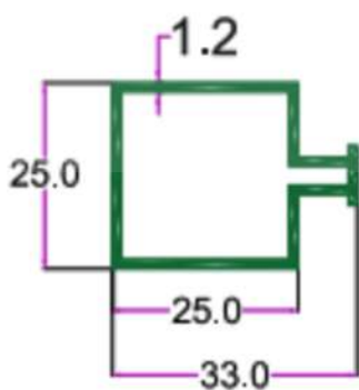
SEC. NO. 2511 WT. 1.330 TO 1.500 KG/12'
