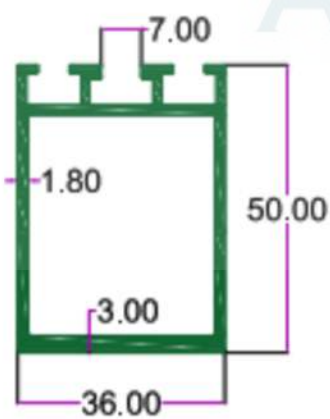
SEC.NO. 4694 WT. 3.210 TO 3.350 KG/12'
