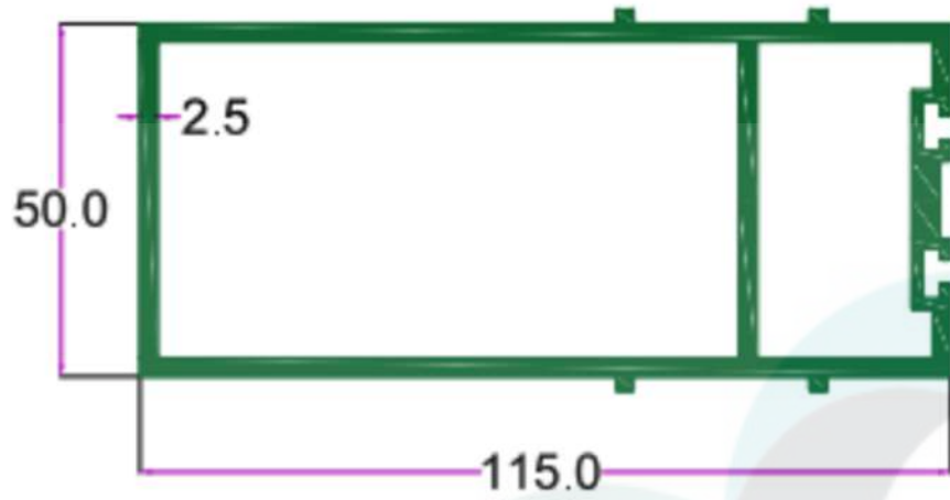
SEC. NO. 2512 WT. 9.370 TO 9.560 KG./12'
