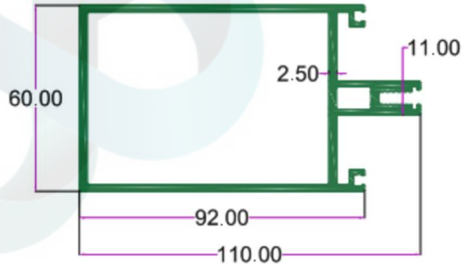
SEC. NO. 4372 WT. 9.270 TO 9.750 KG./12'
