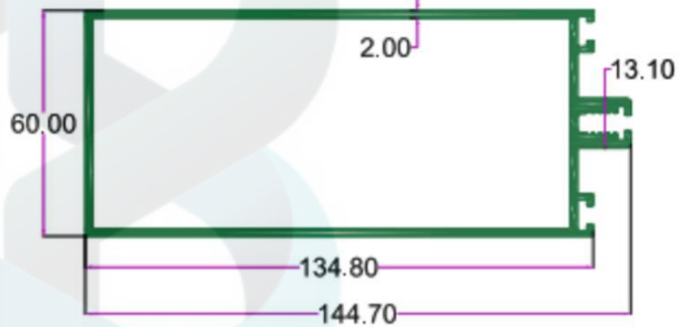
SEC.NO. 5054 WT. 8.720 TO 9.050 KG./ I2'
