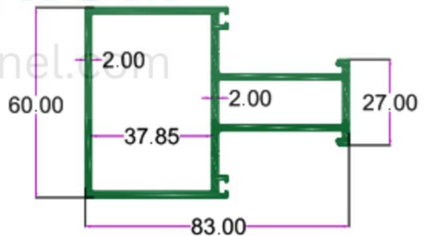
SEC. NO. 4859 WT. 6.200 TO 6.450 KG./12'
