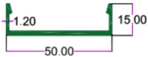
SEC.NO. 5029 WT. 1.370 TO 1.550 KG/12'
