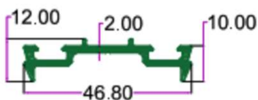
SEC.NO. 5028 WT. 1.330 TO 1.550 KG/12'
