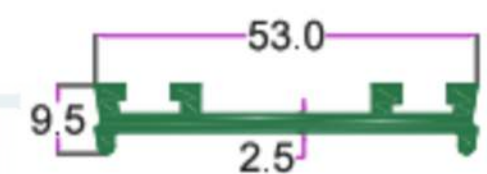
SEC. NO. 2426 WT. 2.300 TO 2.550 KG/15'
