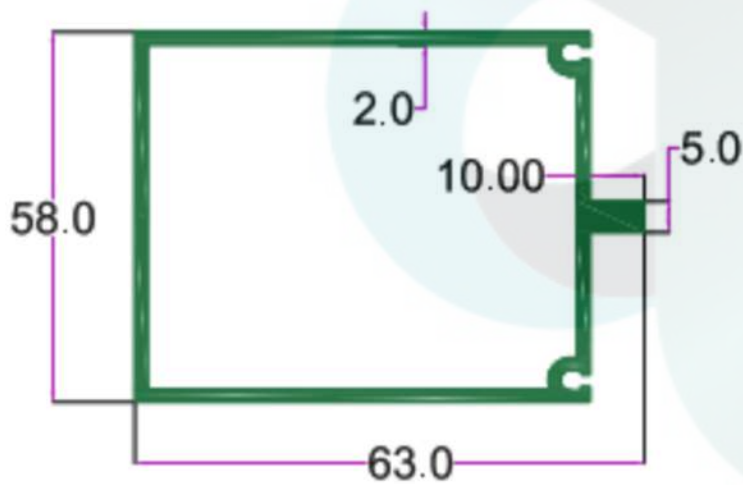
SEC. NO. 2434 WT. 6.500 TO 7.200 KG./15'
