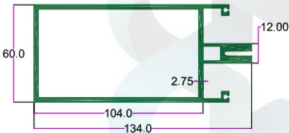
SEC. No. 2438 WT. 12.390 TO 12.600 KG/I2'
