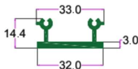
SEC. NO. 2506 WT. 1.460 TO 1.650 KG/I2'
