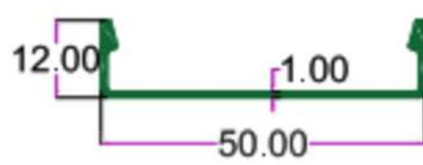
SEC.NO. 5030 WT. 0.800 TO 0.900 KG/12'
