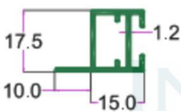
SEC. NO. 2501 WT. 0.940 TO 1.200 KG/I2'
