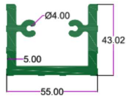
SEC.NO. 5220 WT. 7.850 TO 8.100 KG/12'
