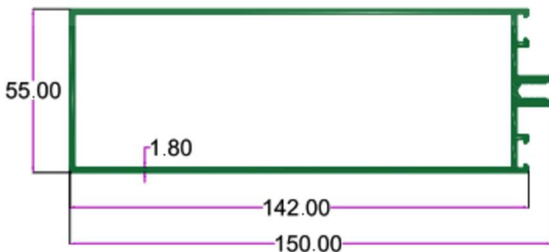
SEC. NO. 3831 WT. 7.500 TO 7.800 KG./12'
