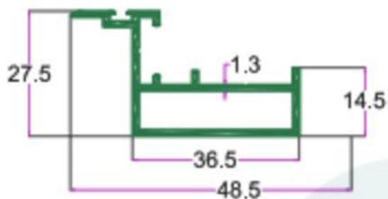
SEC. NO. 2448 WT. 2.370 TO 2.550 KG/15'
