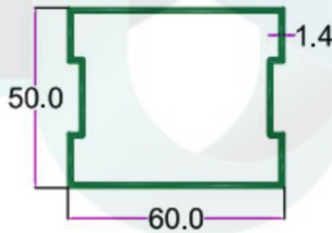
SEC. NO. 3608 WT. 3.000 TO 3.300 KG/12'
