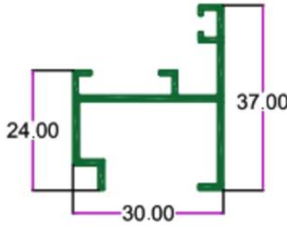
SEC. NO. 3994 WT. 1.300 TO 1.600 KG/I2'
