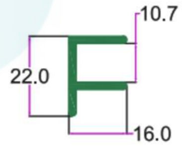
SEC. NO. 2842 WT. 0.850 TO 0.950 KG/I2'
