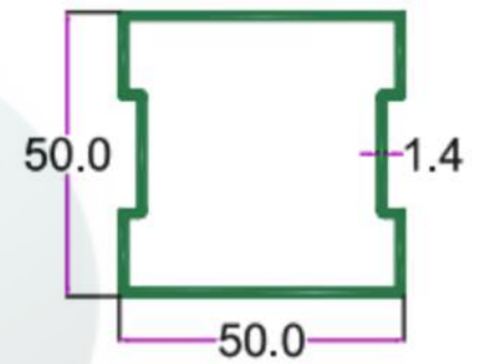
SEC. NO. 3603 WT. 2.700 TO 3.000 KG/12'
