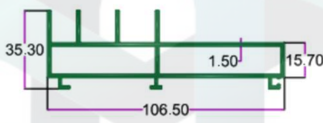
SEC. NO. 4027 WT. 4.900 TO 5.300 KG/I2'
