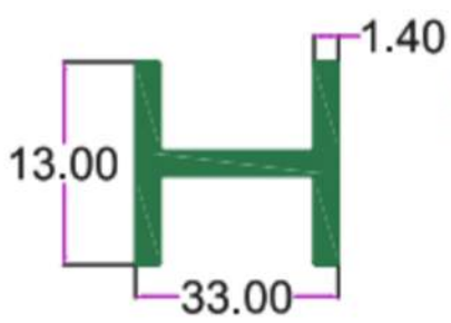
SEC. NO. 533 WT. 1.000 TO 1.200 KG/I2'
