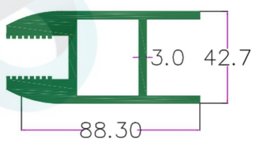
SEC.No. 1758 WT. 10.00 TO 11.00 KG/15'
