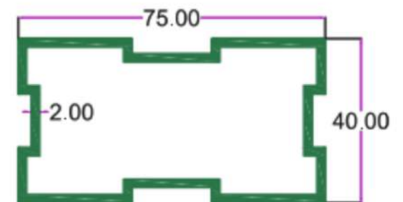
SEC. NO. 3830 WT. 4.90 TO 5.30 KG/12'
