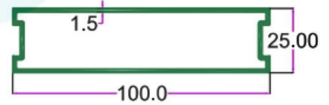
SEC. NO. 3607 WT. 3.600 TO 4.000 KG/12'
