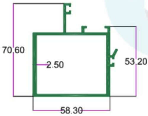
SEC. NO. 4026 WT. 4.700 TO 5.00 KG/I2'
