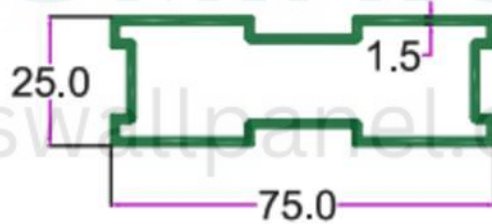
SEC. NO. 3605 WT. 3.000 TO 3.450 KG/12'
