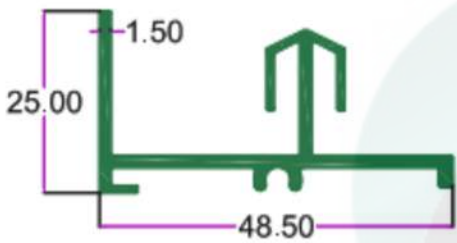
SEC. NO. 3993 WT. 1.750 TO 2.000 KG/I2'
