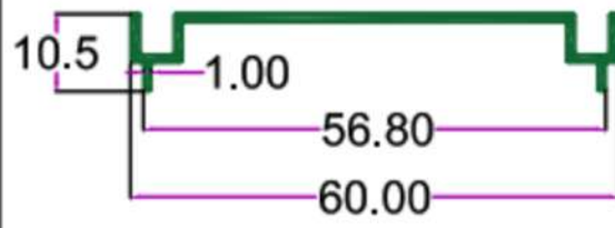
SEC. NO. 3891 WT. 0.890 TO 1.200 KG/12'
