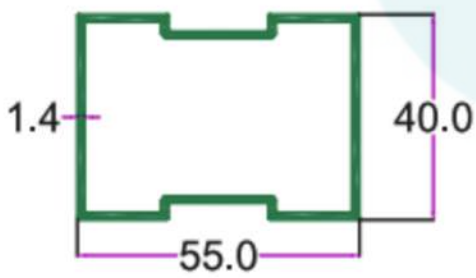
SEC. NO. 3604 WT. 2.600 TO 2.900 KG/12'
