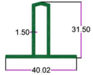
SEC. NO. 4017 WT. 1.500 TO 1.700 KG/I2'
