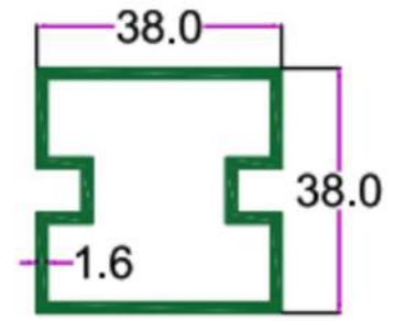
SEC. NO. 3136 WT. 2.745 TO 2.950 KG/12'
