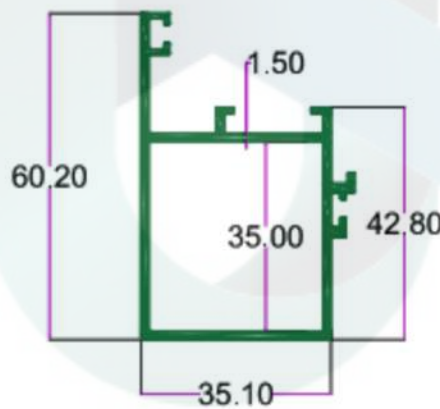
SEC. NO. 4028 WT. 2.800 TO 3.100 KG/I2'
