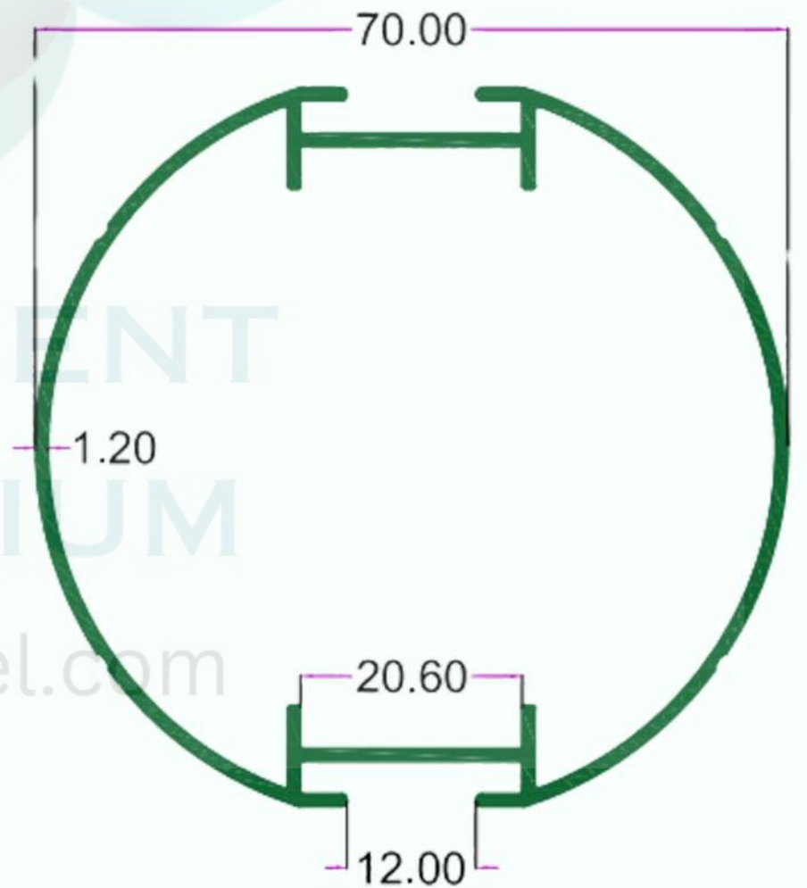
SEC. NO. 4177 WT. 3.100 TO 3.300 KG/12'
