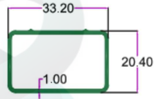
SEC. NO. 4050 WT. 0.990 TO 1.200 KG/12'
