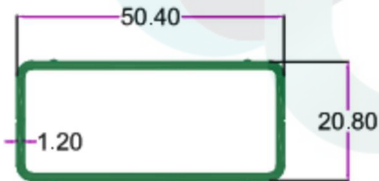
SEC. NO. 4049 WT. 1.340 TO 1.500 KG/12'
