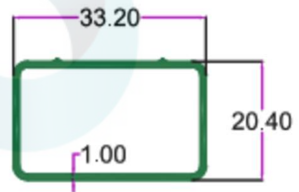
SEC. NO. 4050 WT. 0.990 TO 1.200 KG/12'
