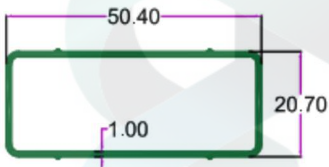
SEC. NO. 4049 WT. 1.340 TO 1.500 KG/12'
