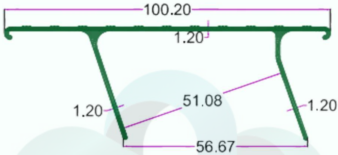
SEC. NO. 4083 WT. 2.200 TO 2.350 KG/12'
