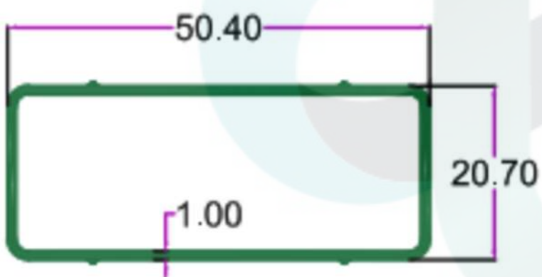
SEC. NO. 4049 WT. 1.340 TO 1.500 KG/12'
