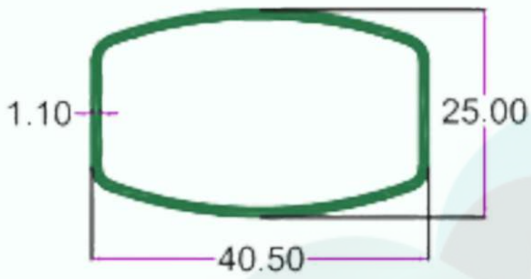
SEC. NO. 4001 WT. 1.200 TO 1.550 KG/12'
