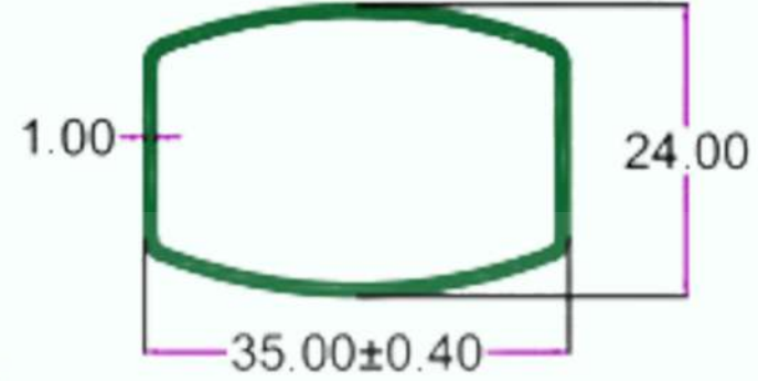
SEC. NO. 4002 WT. 1.000 TO 1.350 KG/12'
