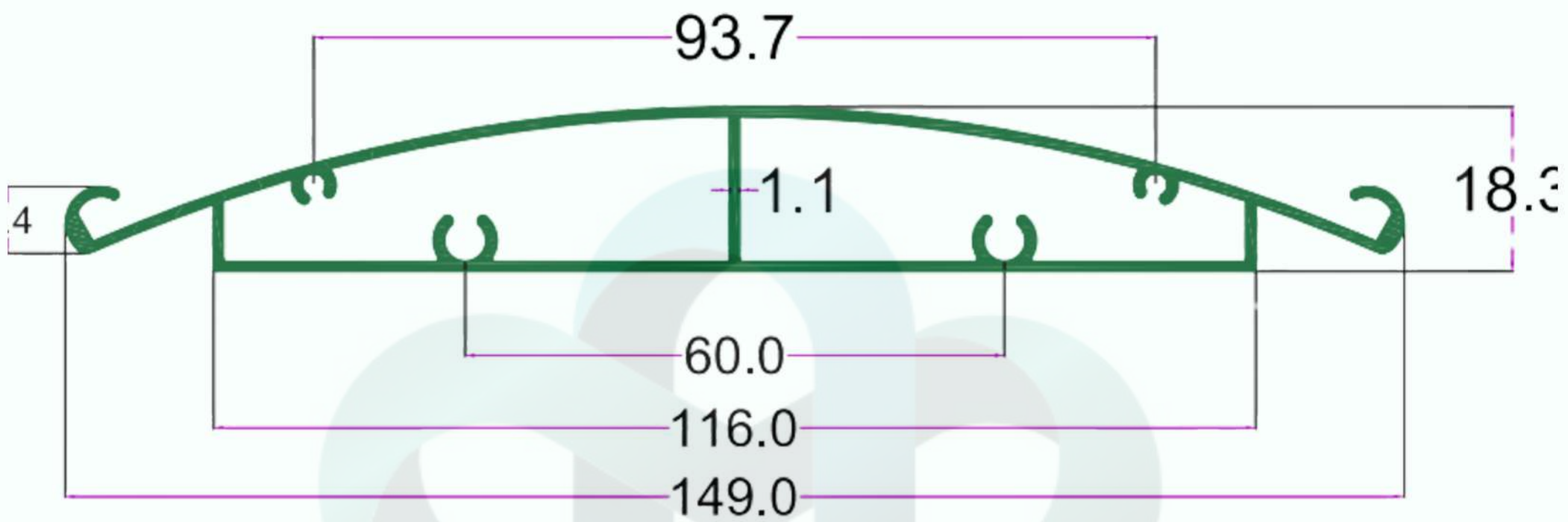
SEC. NO. 1466 WT. 3.929 TO 4.100 KG/12'
