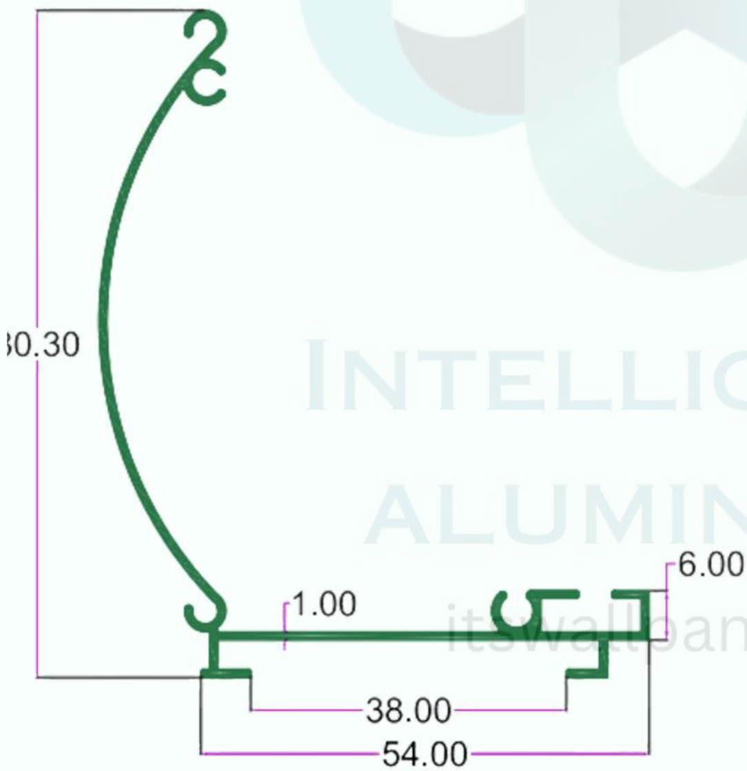
SEC. NO. 1465 WT. 2.140 TO 2.300 KG/12'
