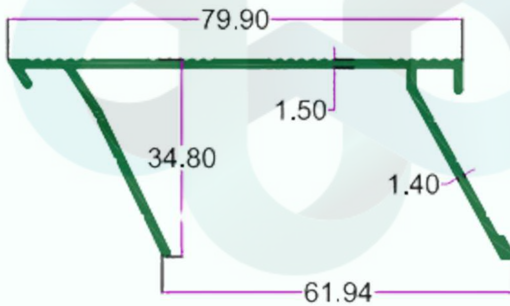
SEC. NO. 4091 WT. 2.250 TO 2.400 KG/12'
