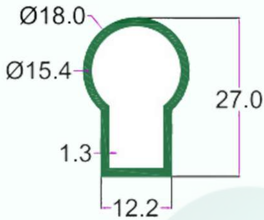
SEC. NO. 3183 WT. 0.900 TO 1.000 KG/12'
