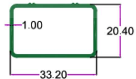
SEC. NO. 4090 WT. 1.000 TO 1.150 KG/12'
