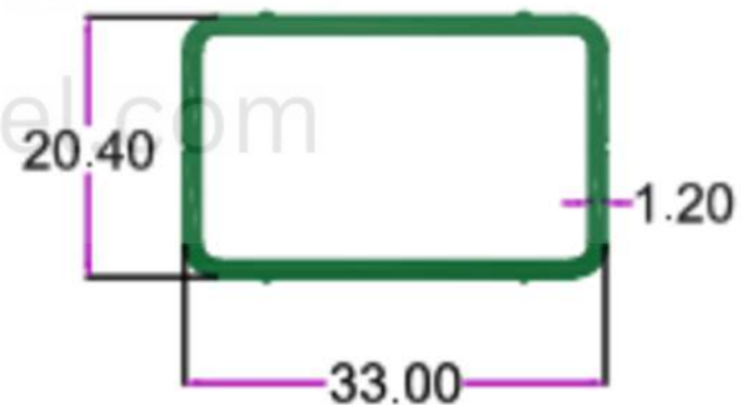
SEC. NO. 4075 WT. 1.150 TO 1.220 KG/12'
