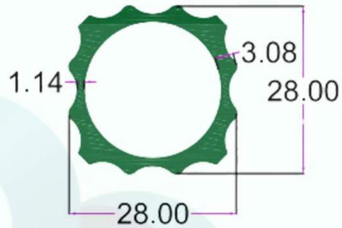
SEC. NO. 5091 WT. 2.220 TO 2.470 KG/12'
