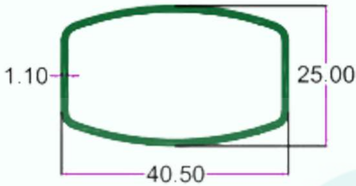
SEC. NO. 4001 WT. 1.200 TO 1.550 KG/12'
