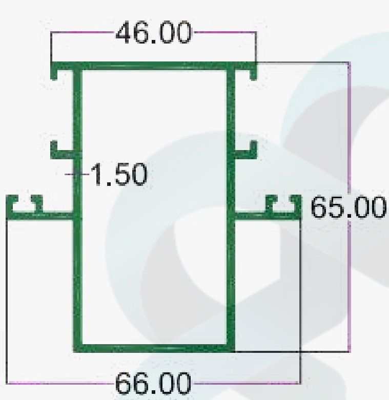
SEC. NO. 4101 WT. 3.920 TO 4.250 KG/12'
