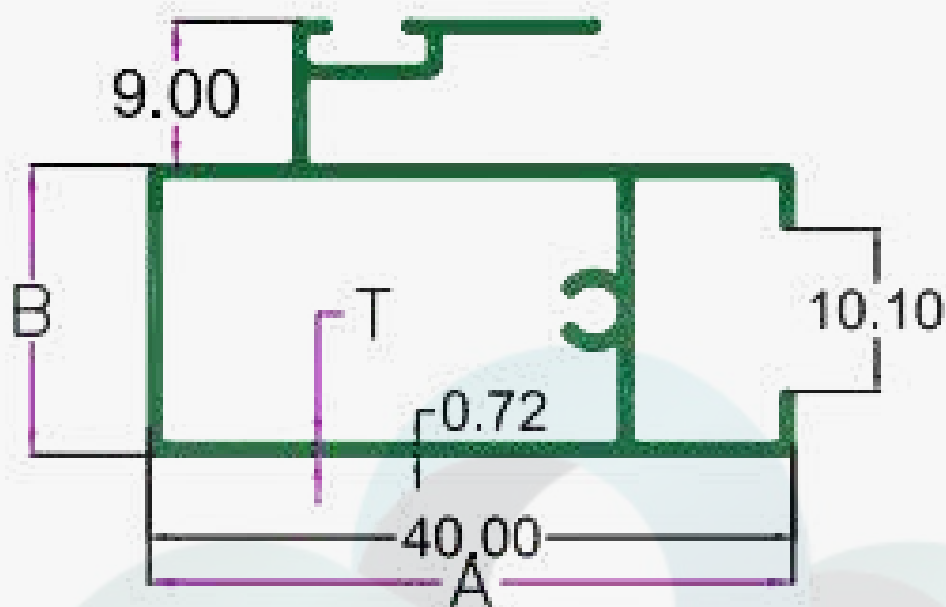
3/4" INTER LOCK
