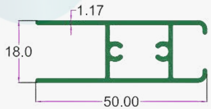
SEC. NO. 1997 WT. 2.000 TO 2.200 KG/15'
