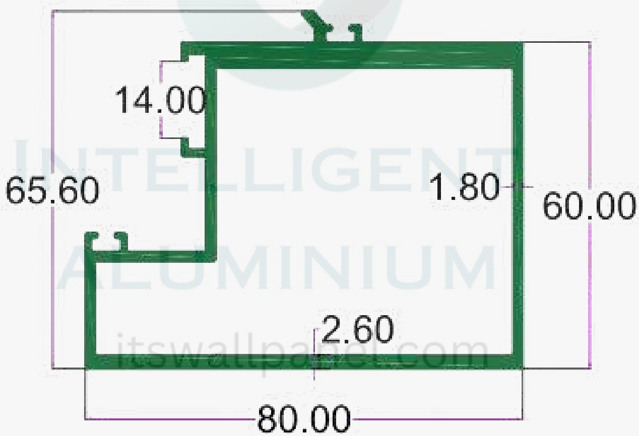
SEC. NO. 4585 WT. 7.530 TO 7.700 KG/12'
