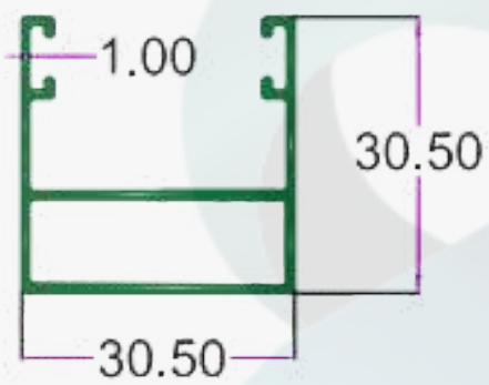
SEC. NO. 1898 WT. 1.400 To 1.600 KG/12'
