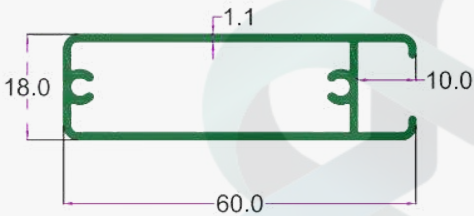
SEC. NO. 1993 WT. 2.250 TO 2.350 KG/12'
