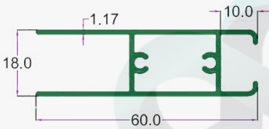
SEC. NO. 1994 WT. 2.700 TO 2.850 KG/15'
