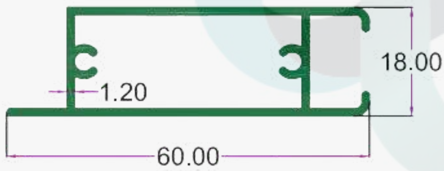
SEC. NO. 1999 WT. 2.390 TO 2.500 KG/15'
