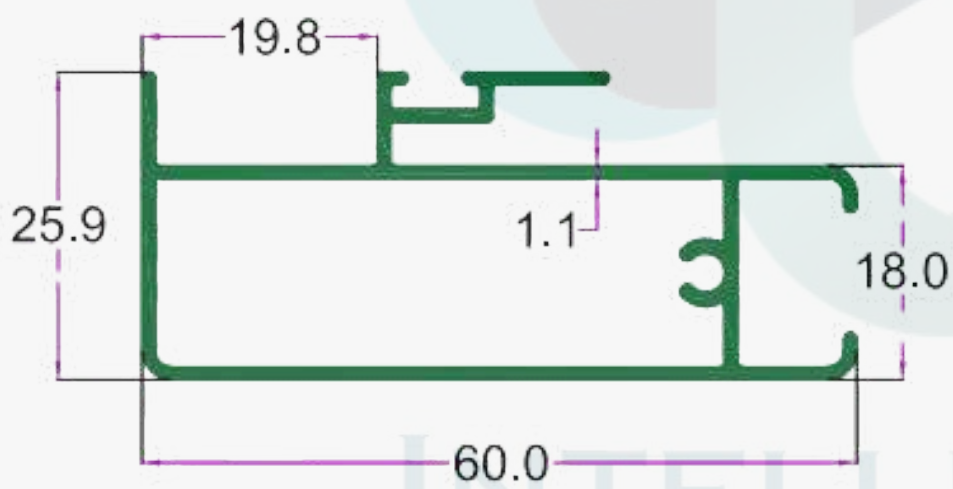
SEC. NO. 1995 WT. 3.150 TO 3.250 KG/15'
