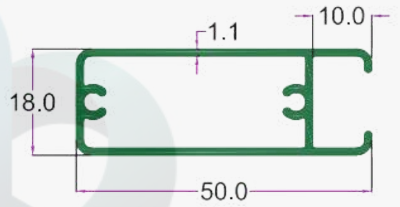
SEC. NO. 1996 WT. 2.000 TO 2.150 KG/15'
