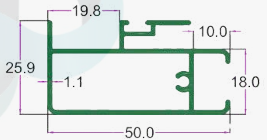
SEC. NO. 1998 WT. 2.450 TO 2.550 KG/15'
