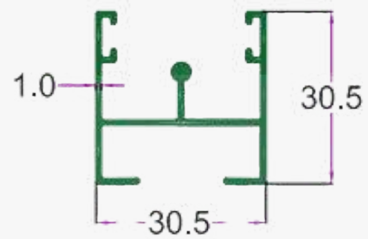
SEC. NO. 1897 WT. 1.200 To 1.400 KG/12'
