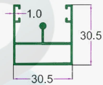
SEC. NO. 1899 WT. 1.550 To 1.750 KG/12'
