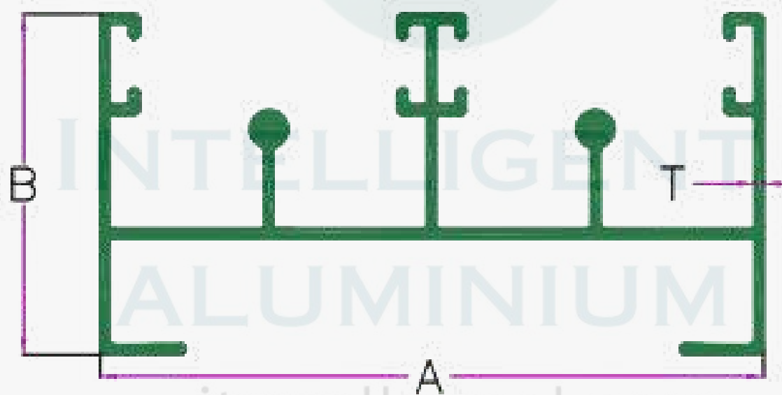
3/4" 2 TRACK BOTTOM
