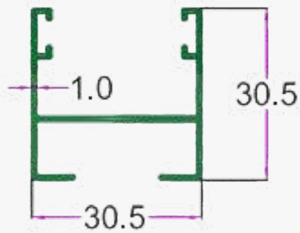
SEC. NO. 1896 WT. 1.100 To 1.300 KG/12'
