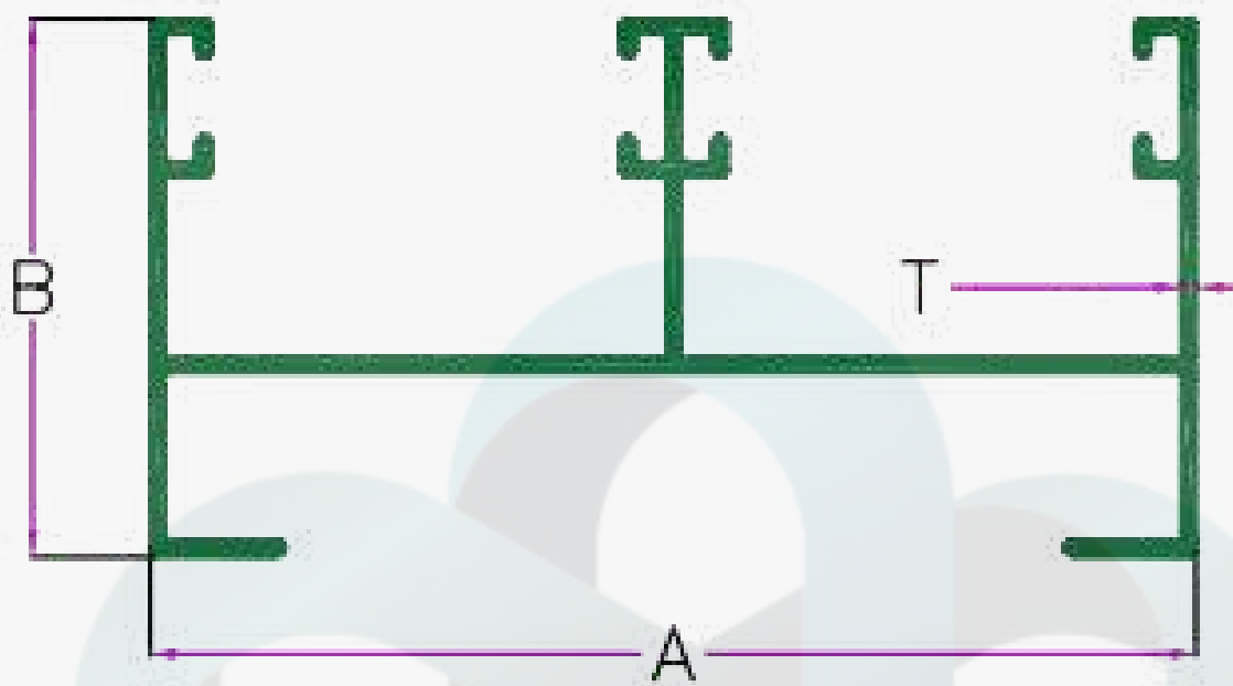
3/4" 2 TRACK TOP
