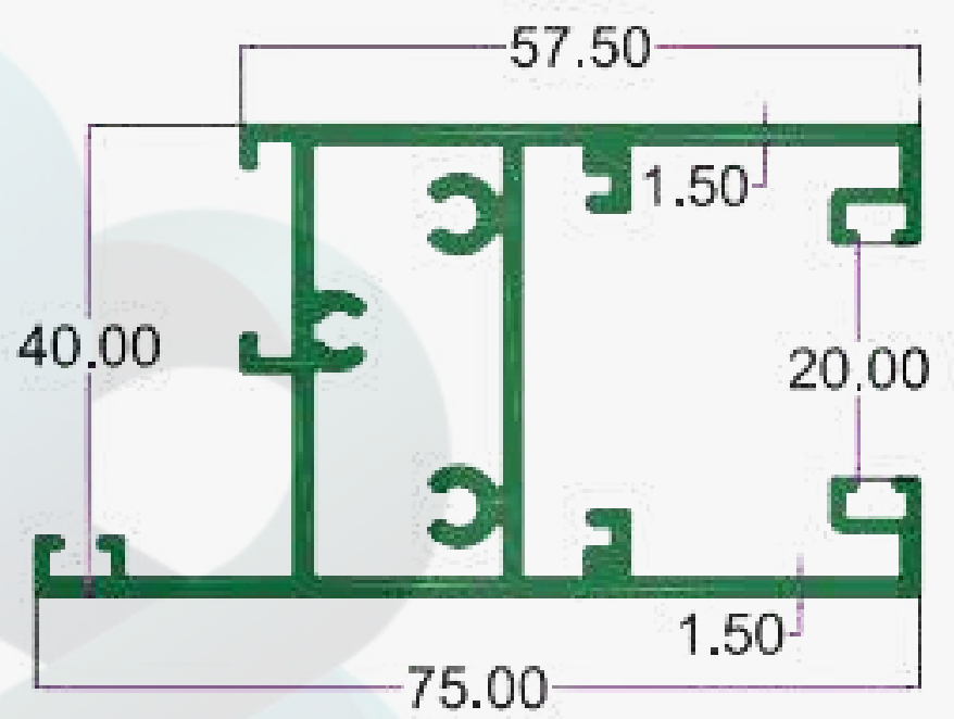
SEC. NO. 4586 WT. 4.580 TO 4.900 KG/12'
