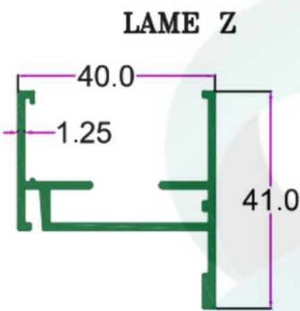
SEC. NO. 2054 WT. 2.900 TO 3.100 KG/15'
