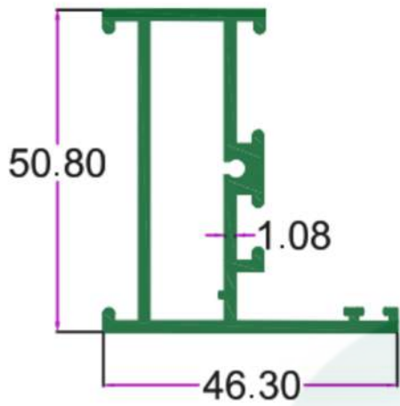
SEC. NO. 3778 WT. 3.600 TO 3.800 KG/12'
