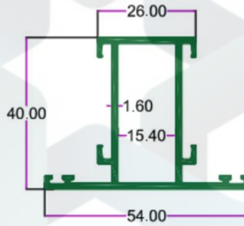
SEC. NO. 4766 WT. 2.800 TO 3.000 KG/12'
