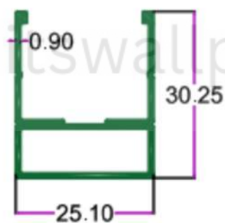
SEC.NO. 4993 WT. 1.125 TO 1.250 KG/12'
