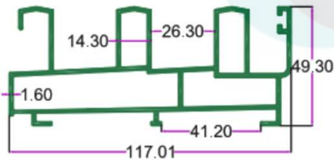
SEC. NO. 3320 WT. 8.000 TO 8.250 KG/12'
