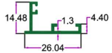
SEC. NO. 2065 WT. 1.000 TO 1.200 KG/12'
