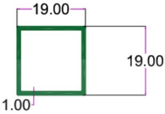
SEC.NO. 4346 WT. 0.700 TO 0.850 KG/12'
