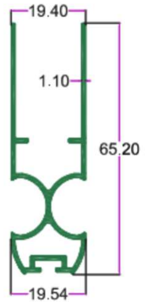
SEC.NO. 4778 WT. 2.000 TO 2.150 KG/12'
