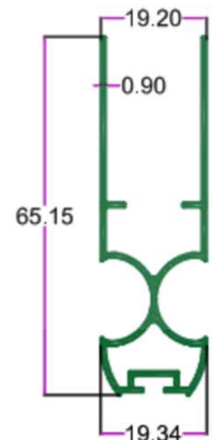
SEC.NO. 4994 WT. 1.635 TO 1.780 KG/12'
