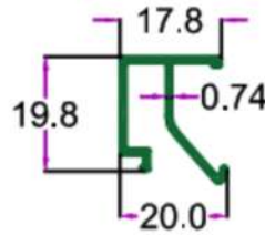
SEC. No. 3285 WT. 0.730 TO 0.850 KG/12'
