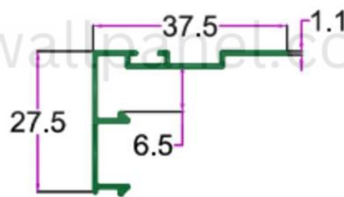
SEC. NO. 3312 WT. 0.940 TO 1.110 KG./12'
