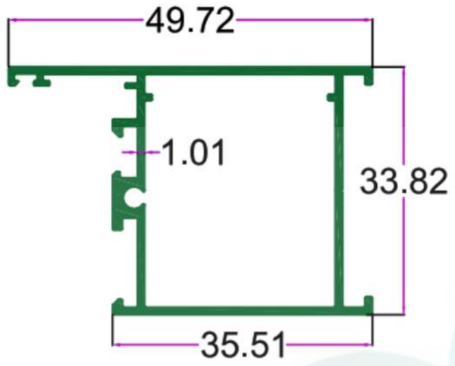
SEC.NO. 4771 WT. 3.320 TO 3.520 KG/I2'
