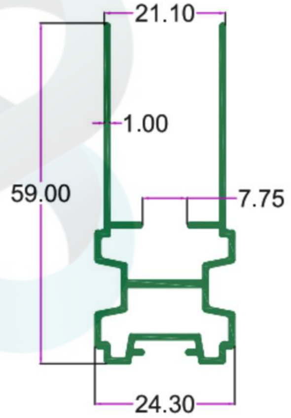
SEC.NO. 4813 WT. 1.950 TO 2.150 KG/12'
