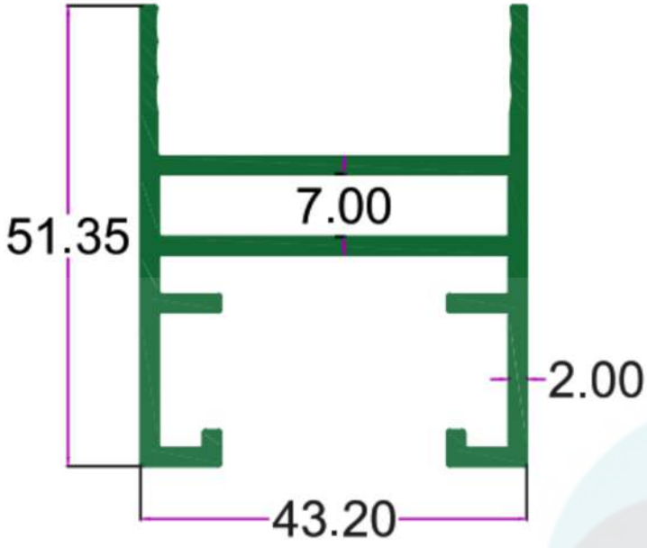
SEC.NO. 5238 WT. 4.118 TO 4.368 KG/I2'
