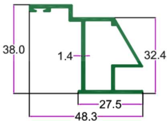
SEC. NO. 3458 WT. 1.900 TO 2.200 KG/12'
