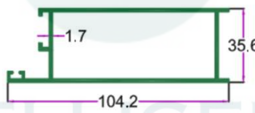
SEC. NO. 2064 WT. 4.647 TO 8.000 KG/12'
