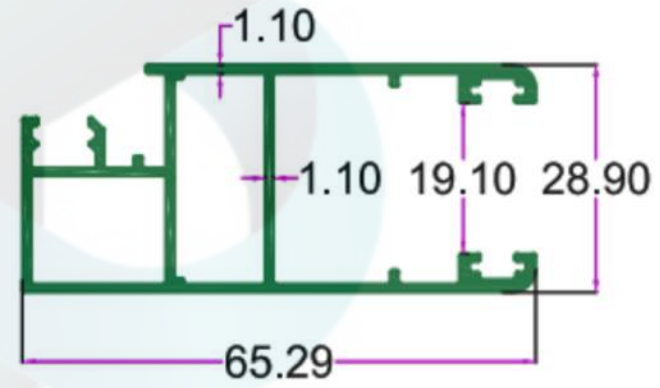
SEC.NO. 4925 WT. 2.750 TO 3.050 KG/12'
