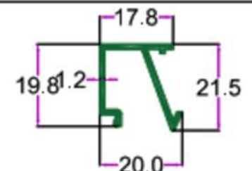
SEC. NO. 3340 WT. 0.70 TO 0.850 KG/I2'
