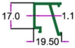
SEC. NO. 3518 WT. 0.700 TO 0.800 KG/12'
