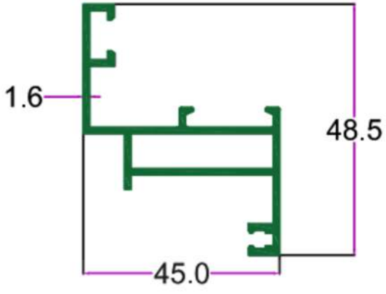
SEC. NO. 2208 WT. 2.500 TO 3.500 KG/15'
