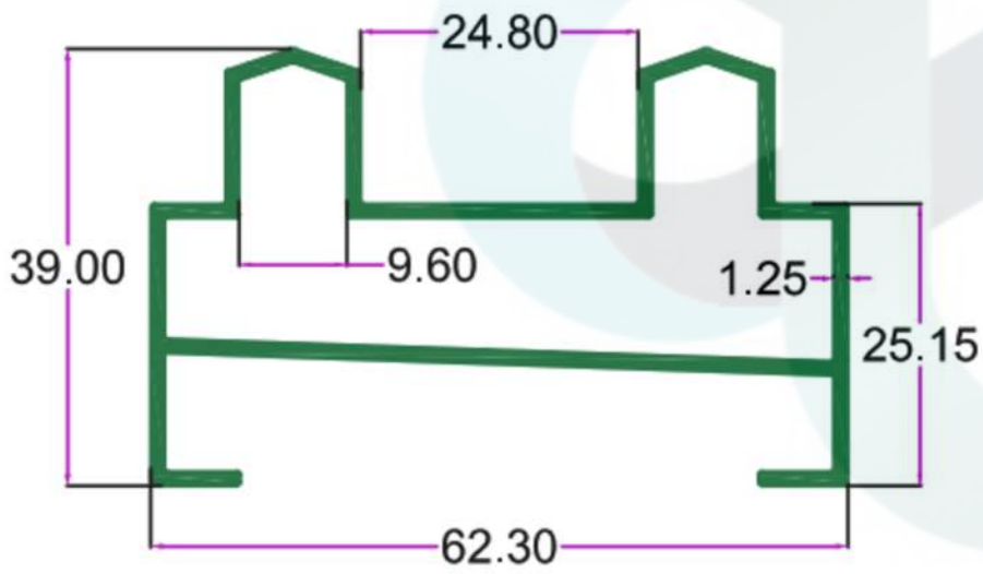
SEC. NO. 4854 WT. 2.870 TO 3.080 KG/12'
