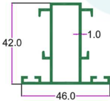
MULLION
