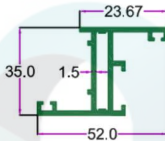
SEC. NO. 3516 WT. 2.200 TO 2.500 KG/12'
