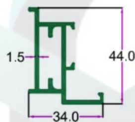
SEC. NO. 3261 WT. 2.026 TO 2.400 KG/12'
