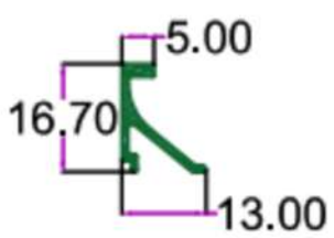
SEC. NO. 4717 WT. 0.420 TO 0.550 KG/I2'
