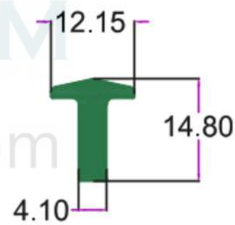
SEC.NO. 4838 WT. 0.750 TO 0.900 KG/I2'
