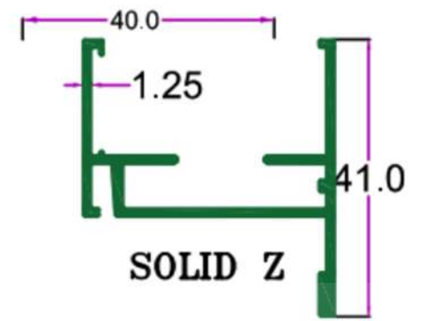
SEC. NO. 2053 WT. 1.700 TO 1.900 KG/12'
