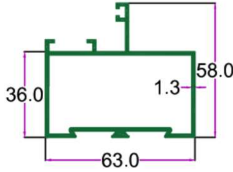
SEC. NO. 3530 WT. 3.100 TO 3.500 KG/12'
