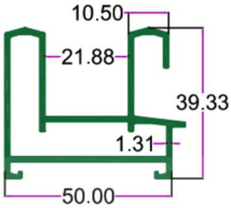
SEC.NO. 4845 WT. 3.650 TO 3.870 KG/12'
