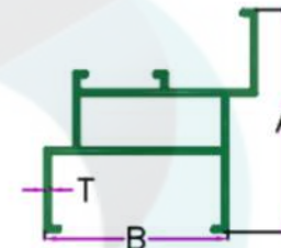
Z BOX SECTION
