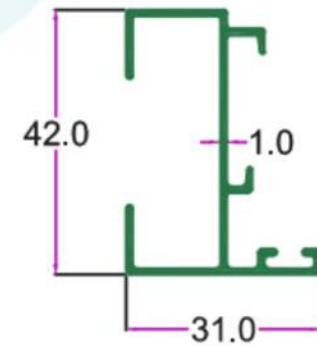
LAME-Z
