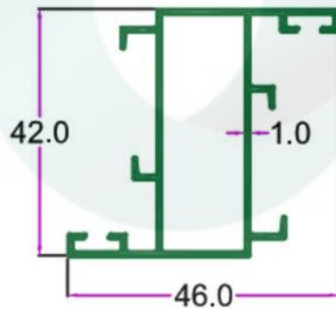
HOLLOW-Z
