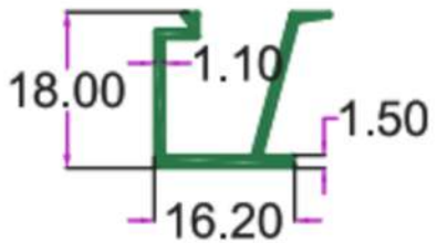
SEC.NO. 4893 WT. 0.580 TO 0.680 KG/12'
