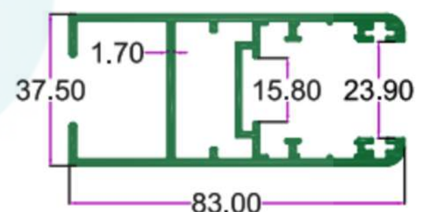
SEC. NO. 4748 WT. 5.240 TO 5.500 KG/I2'
