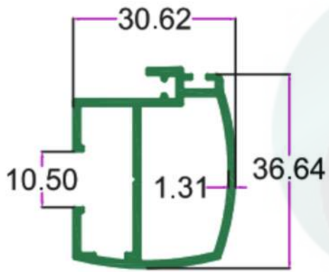
SEC.NO. 4844 WT. 2.630 TO 2.850 KG/12'
