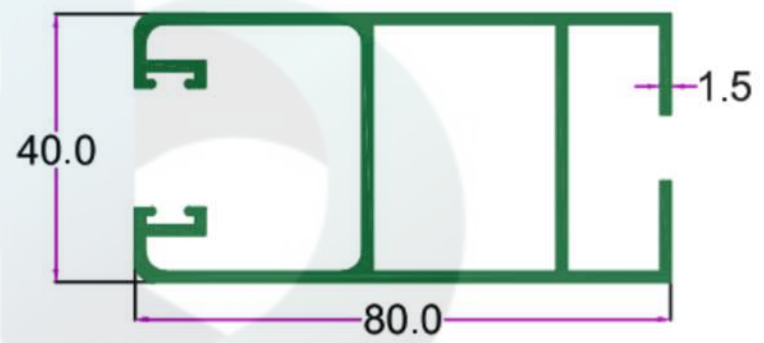
SEC. NO. 2804 WT. 4.500 TO 5.000 KG/12'
