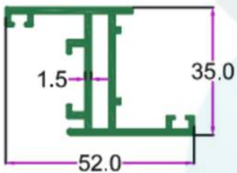
SEC. NO. 3517 WT. 2.300 TO 2.600 KG/12'
