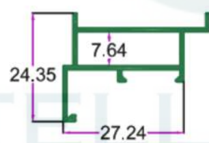
SEC. NO. 2116 WT. 1.800 TO 2.000 KG/12'
