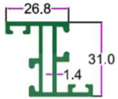
SEC. NO. 2180 WT. 1.900 TO 2.000 KG/12'
