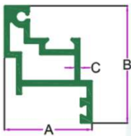
SEC. NO. 2180 WT. 1.900 TO 2.000 KG/12'
