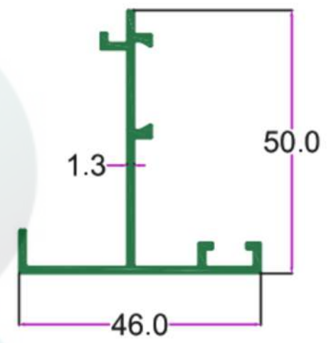
SEC. NO. 3609 WT. 1.600 TO 1.800 KG/12'
