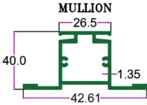
SEC. NO. 2051 WT. 3.900 TO 4.200 KG/15'
