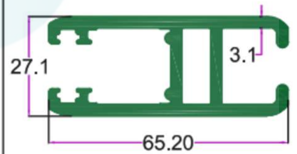
SEC. NO. 3695 WT. 5.750 TO 6.100 KG/12'
