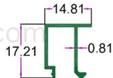
SEC. NO. 5007 WT. 0.940 TO 1.100 KG/12'
