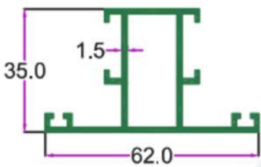
SEC. NO. 3515 WT. 2.300 TO 2.600 KG/12'
