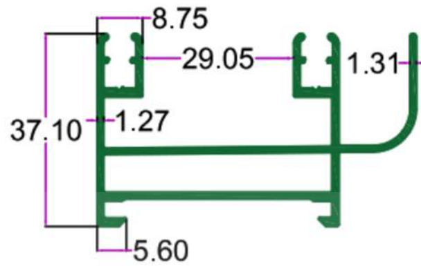
SEC.NO. 4843 WT. 4.180 TO 4.400 KG/12'
