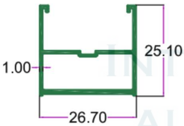
SEC.NO. 5214 WT. 1.280 TO 1.530 KG/12'
