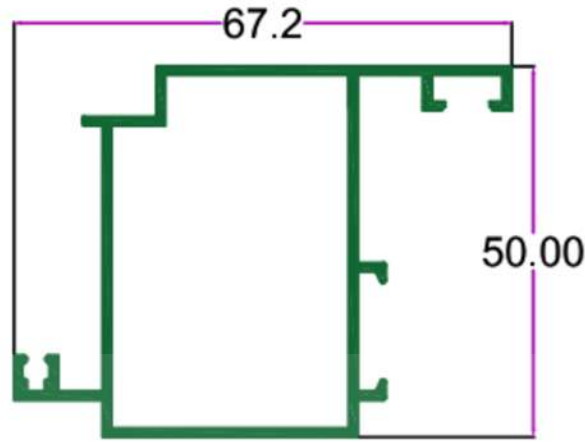
SEC. NO. 2212 WT. 5.900 TO 6.200 KG/15'
