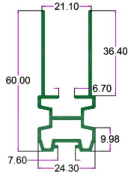
SEC.NO. 4434 WT. 1.930 TO 2.1500 KG/12'
