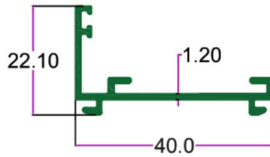
SEC. NO. 3463 WT. 0.920 TO 1.030 KG/12'
