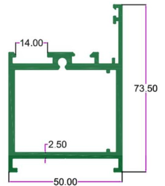
SEC. NO. 5211 WT. 5.530 TO 5.780 KG/12'
