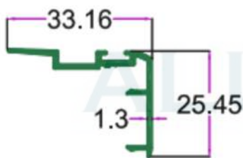
SEC.NO. 3336 WT. 0.690 TO 0.800 KG/12'
