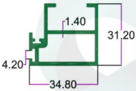
SEC.NO. 5123 WT. 2.110 TO 2.360 KG/12'
