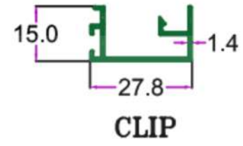
SEC. NO. 2164 WT. 1.050 TO 1.240 KG/15'
