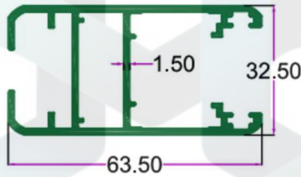
SEC.NO. 3319 WT. 3.850 TO 4.050 KG/12'
