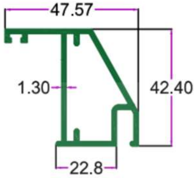
SEC. NO. 2181 WT. 1.900 TO 2.200 KG/12'
