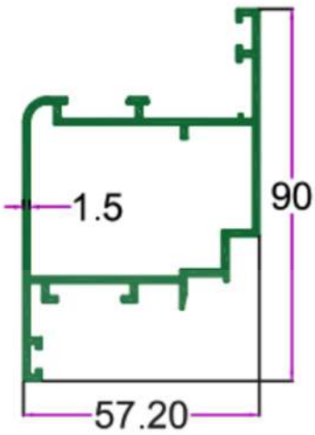
SEC. NO. 3940 WT. 4.400 TO 4.80 KG/12'
