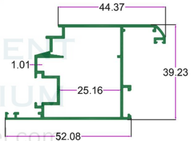
SEC. NO. 4774 WT. 5.150 TO 5.400 KG/12'
