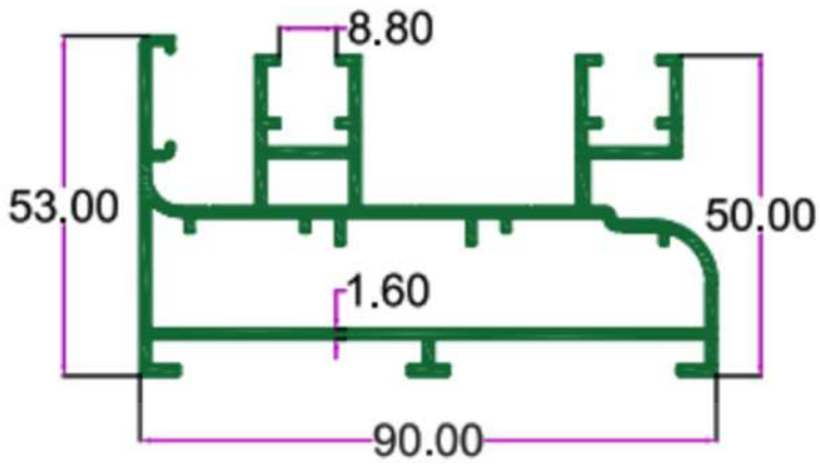
SEC. NO. 4706 WT. 6.700 TO 6.950 KG/I2'
