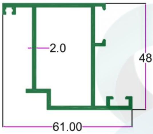
SEC. NO. 2215 WT. 4.550 TO 4.850 KG/15'
