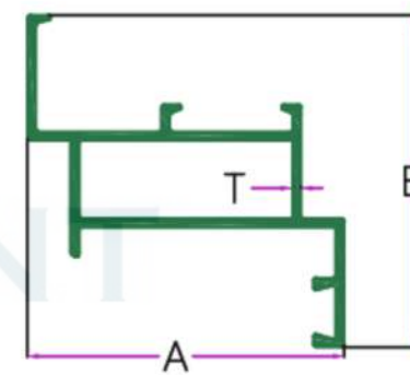
Z HOLLOW SECTION
