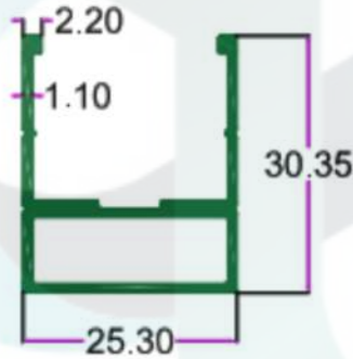
SEC.NO. 4777 WT. 1.340 TO 1.450 KG/12'
