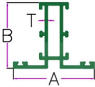
MULLION SECTION (H)
