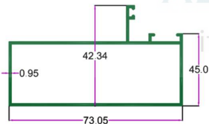
SEC. No. 3286 WT. 4.600 TO 4.900 KG/12'
