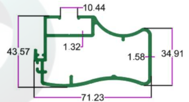
SEC.NO. 4848 WT. 4.880 TO 5.130 KG/12'
