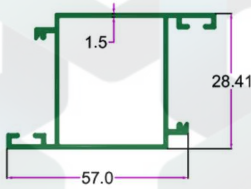
SEC. NO. 2204 WT. 2.600 TO 3.100 KG/15'
