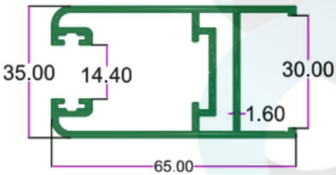
SEC. NO. 4797 WT. 3.950 TO 4.150 KG/12'
