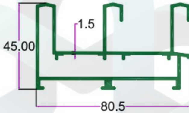
SEC. NO. 3311 WT. 5.200 TO 5.400 KG/12'
