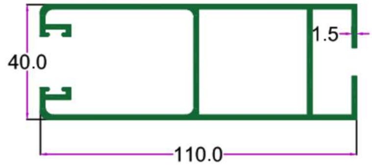
SEC. NO. 2802 WT. 5.400 TO 5.900 KG/12'
