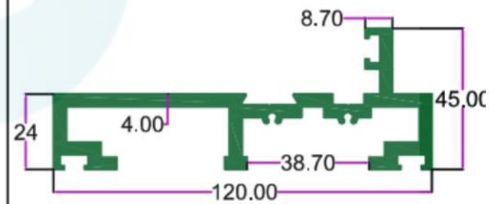
SEC. NO. 3610 WT. 9.500 TO 10.600 KG/12'
