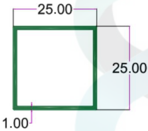
SEC.NO. 4347 WT. 0.900 TO 1.050 KG/12'
