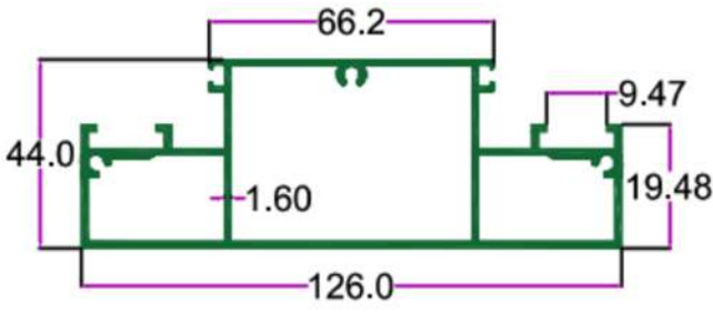
SEC. NO. 3527 WT. 7.100 TO 7.900 KG/12'
