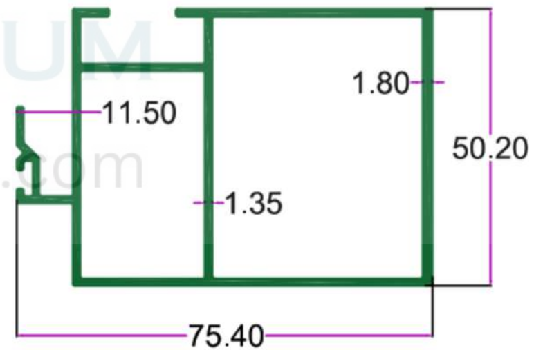
SEC. NO. 4853 WT. 4.360 TO 4.600 KG/12'
