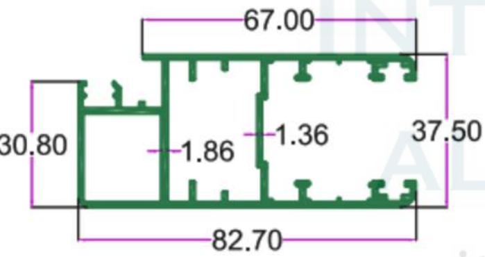
SEC. NO. 4711 WT. 4.820 TO 5.050 KG/I2'
