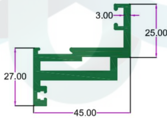
SEC. NO. 3613 WT. 4.700 TO 5.150 KG/12'
