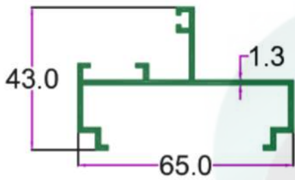
SEC. NO. 3528 WT. 2.050 TO 2.300 KG/12'
