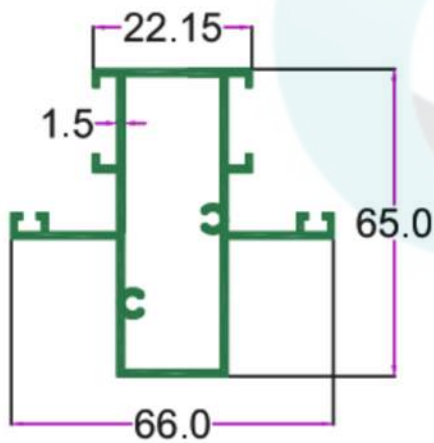
SEC. NO. 3531 WT. 3.800 TO 4.200 KG/12'
