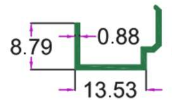
SEC. NO. 3526 WT. 0.630 TO 0.710 KG/12'
