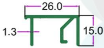
SEC. NO. 2203 WT. 1.050 TO 1.400 KG/15'
