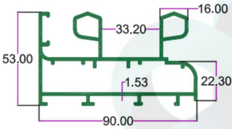
SEC. NO. 4712 WT. 6.440 TO 6.620 KG/I2'
