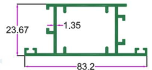
SEC. NO. 2067 WT. 3.622 TO 3.800 KG/12'
