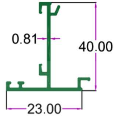
SEC. NO. 4270 WT. 1.200 TO 1.400 KG./ 12'
