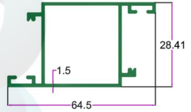
SEC. NO. 2205 WT. 3.250 TO 3.750 KG/15'
