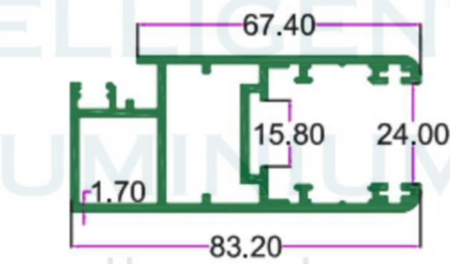
SEC. NO. 4747 WT. 5.700 TO 5.950 KG/I2'
