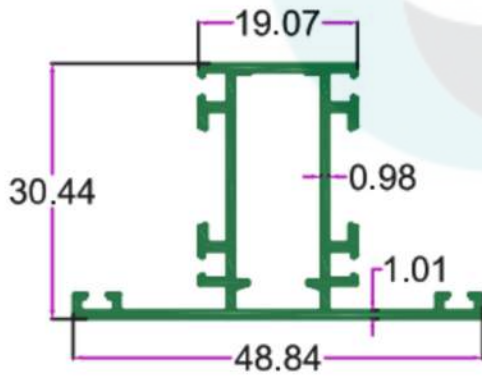
SEC. NO. 4930 WT. 3.720 TO 3.980 KG/12'
