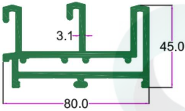
SEC. NO. 3694 WT. 9.60 TO 10.60 KG/12'
