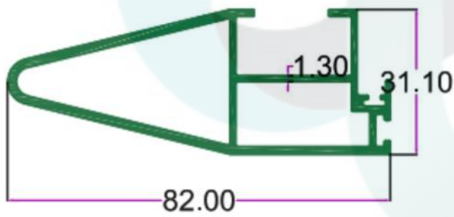
SEC.NO. 5119 WT. 3.915 TO 4.165 KG/12'
