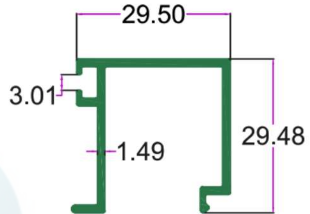
SEC.NO. 5114 WT. 1.480 TO 1.730 KG/12'
