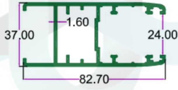
SEC. NO. 4709 WT. 4.610 TO 4.850 KG/I2'
