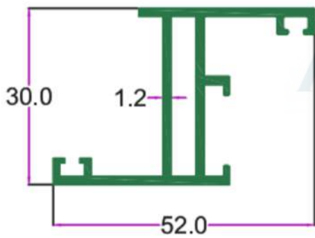
SEC. NO. 3523 WT. 1.650 TO 1.850 KG / 12'
