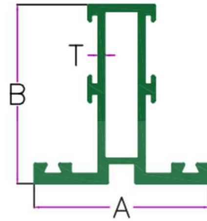
MULLION SECTION (J)
