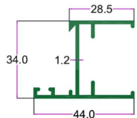
SEC. No. 3372 WT. 1.550 TO 1.850 KG/12'
