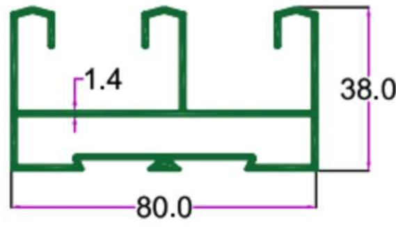
SEC. NO. 3316 WT. 4.290 TO 4.500 KG/12'
