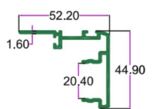
SEC. NO. 4710 WT. 2.420 TO 2.610 KG/I2'
