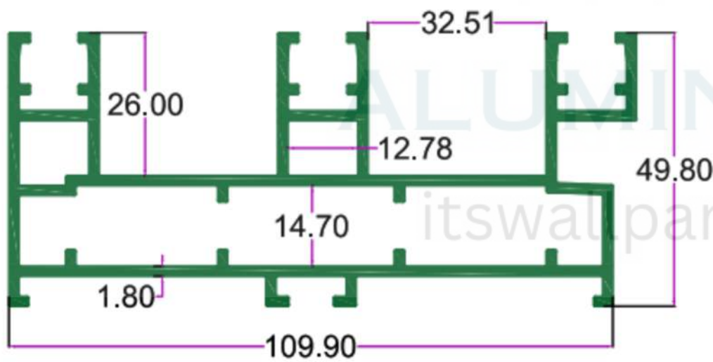
SEC.NO. 4740 WT. 9.020 TO 9.300 KG/12'
