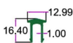
SEC. NO. 4705 WT. 0.550 TO 0.650 KG/I2'
