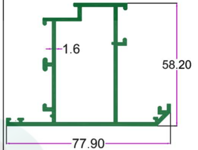
SEC. NO. 3780 WT. 4.200 TO 4.500 KG/12'
