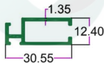
SEC.NO. 5118 WT. 0.995 TO 1.245 KG/12'
