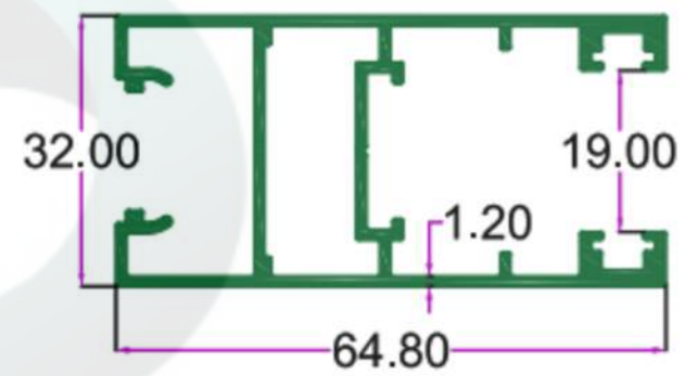
SEC.NO. 4892 WT. 3.360 TO 3.560 KG/12'
