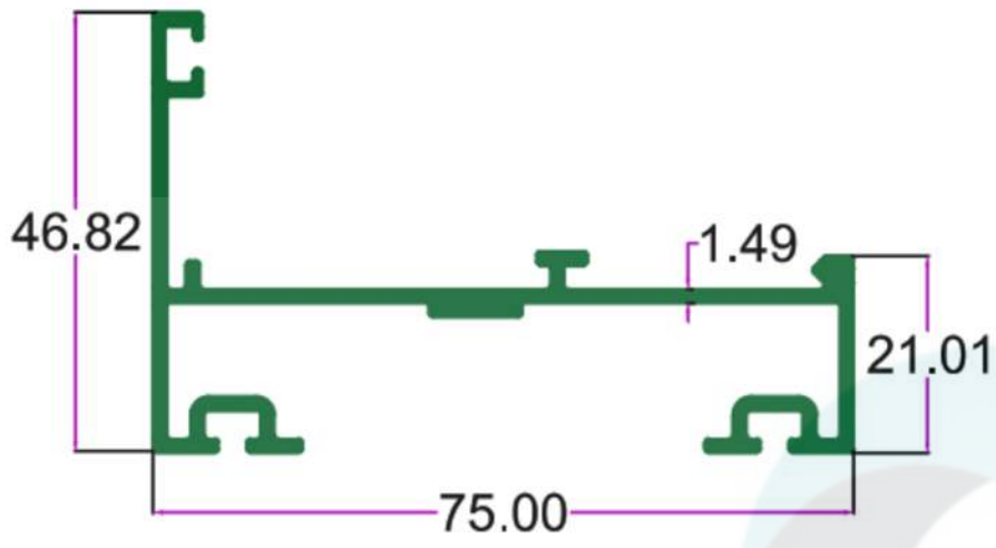
SEC.NO. 5113 WT. 3.340 TO 3.590 KG/12'
