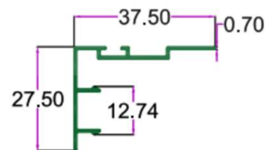
SEC. NO. 4421 WT. 0.600 TO 0.850 KG/12'
