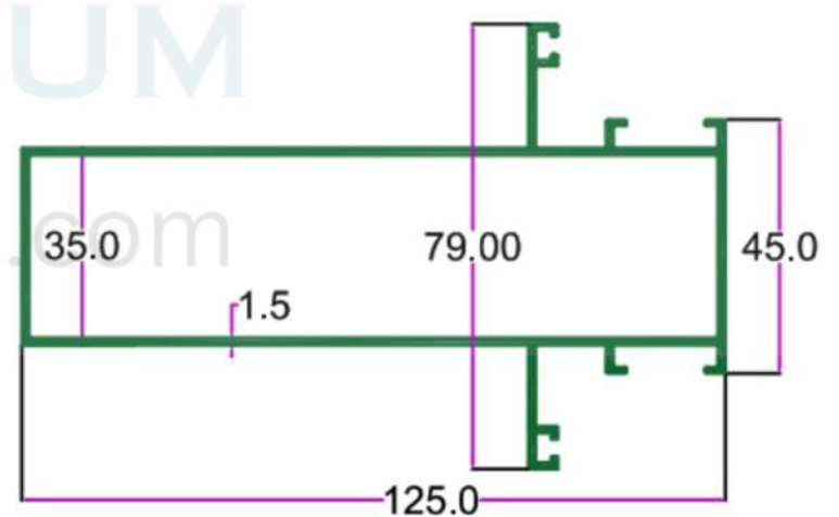
SEC. NO. 3514 WT. 5.600 TO 6.200 KG/12'
