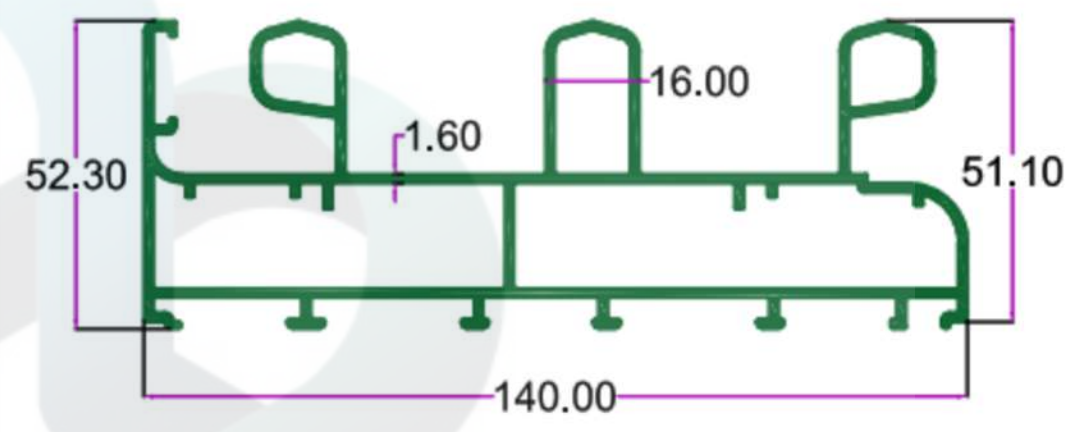
SEC. NO. 4713 WT. 9.810 TO 10.120 KG/I2'
