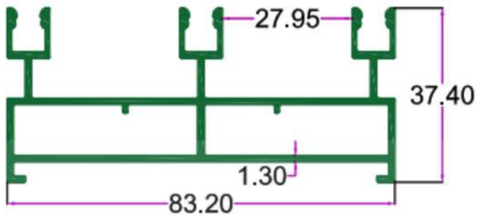
SEC.NO. 5121 WT. 2.810 TO 3.060 KG/12'
