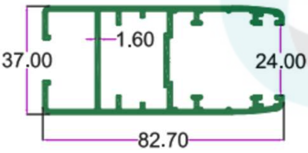
SEC. NO. 4708 WT. 4.860 TO 5.050 KG/I2'
