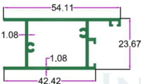
SEC. NO. 3519 WT. 3.600 TO 4.000 KG/12'
