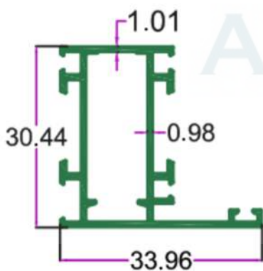
SEC. NO. 4929 WT. 3.225 TO 3.500 KG/12'
