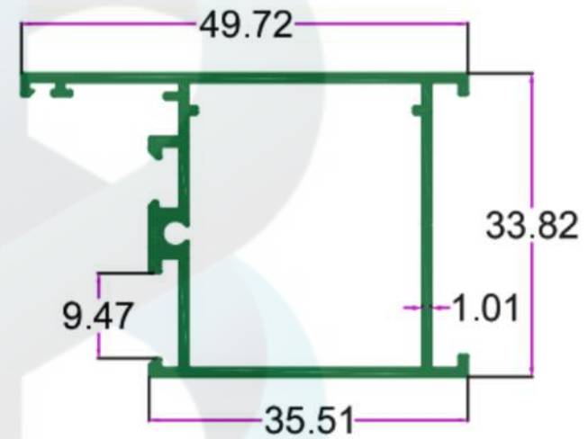
SEC. NO. 4771 WT. 3.320 TO 3.520 KG/12'
