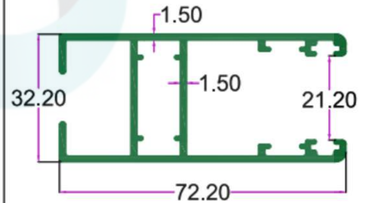
SEC.NO. 4351 WT. 3.760 TO 3.950 KG/12'
