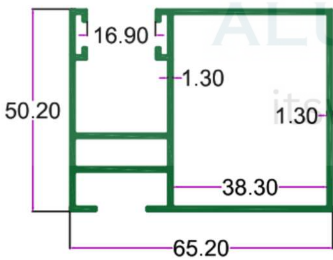
SEC. NO. 4852 WT. 3.900 TO 4.120 KG/12'
