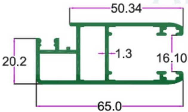
SEC. NO. 3331 WT. 3.100 TO 3.400 KG/12'
