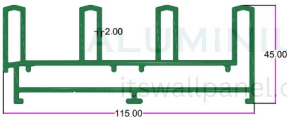
SEC. NO. 5131 WT. 9.870 TO 10.12 KG/12'
