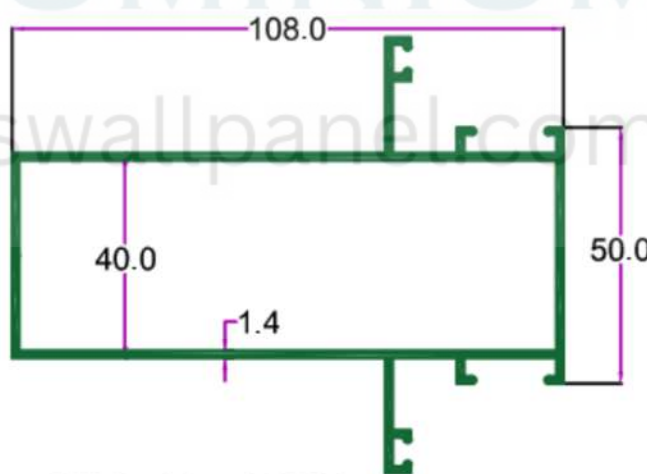
SEC. No. 3287 WT. 5.240 TO 5.500 KG/12'
