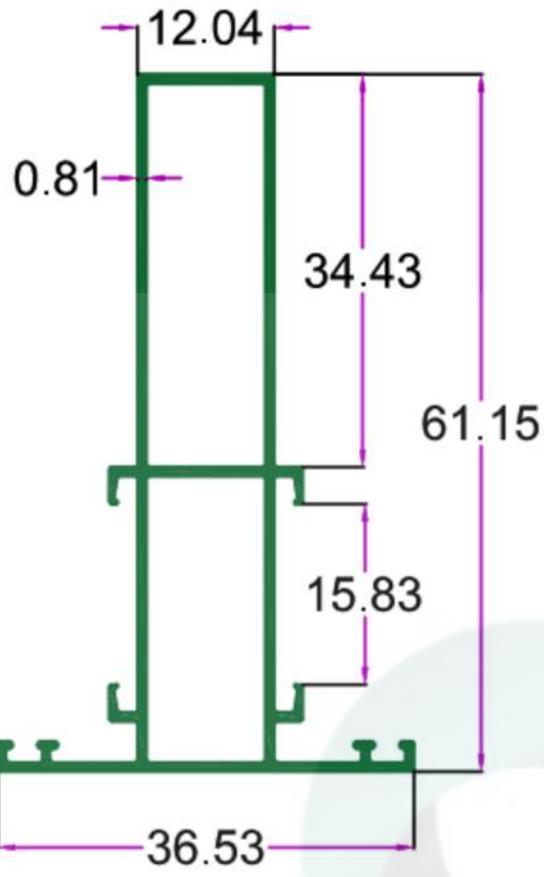
SEC. NO. 4271 WT. 3.500 TO 3.800 KG./ 12'
