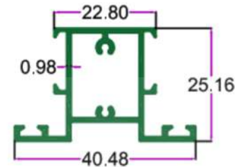
SEC. NO. 3263 WT. 2.906 TO 3.212 KG/12'
