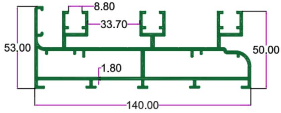
SEC. NO. 4707 WT. 10.540 TO 10.800 KG/I2'
