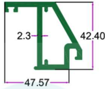
SEC. NO. 2182 WT. 3.950 TO 4.100 KG/15'
