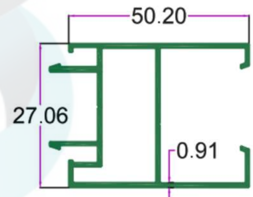
SEC. NO. 3783 WT. 2.850 TO 3.00 KG/12'
