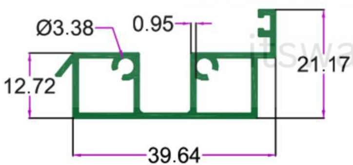
SEC. NO. 5010 WT. 2.900 TO 3.100 KG/12'
