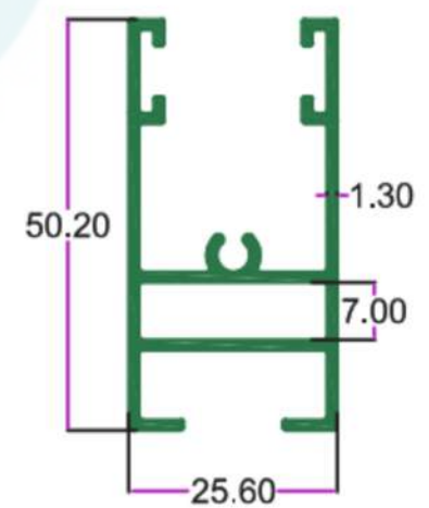
SEC.NO. 4965 WT. 2.410 TO 2.600 KG/12'
