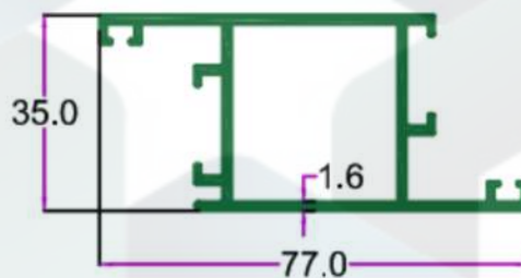
SEC. NO. 3520 WT. 3.100 TO 3.500 KG/12'
