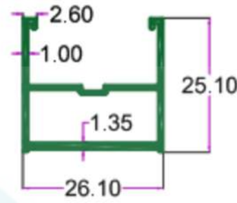
SEC.NO. 4432 WT. 1.100 TO 1.300 KG/12'
