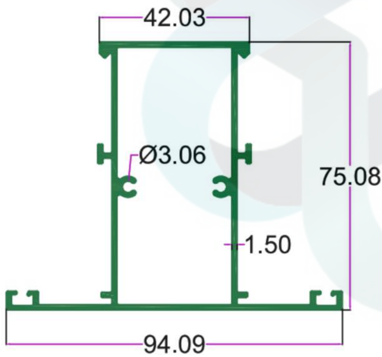
SEC.NO. 5116 WT. 5.270 TO 5.520 KG/12'
