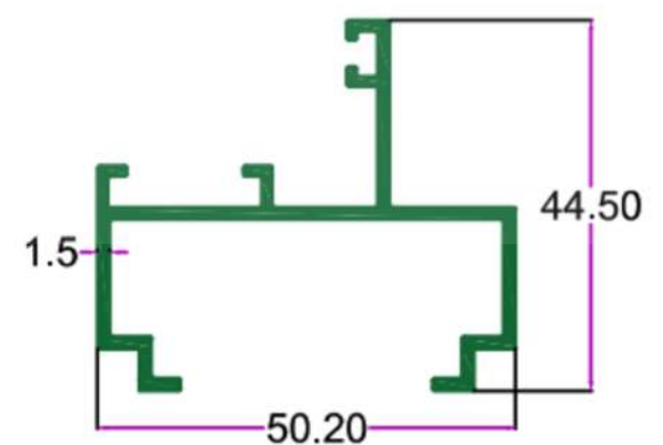
SEC. NO. 3650 WT. 2.200 TO 2.500 KG/12'
