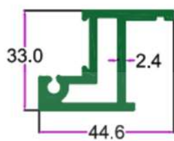
SEC. No. 3154 WT. 3.200 TO 3.540 KG/12'
