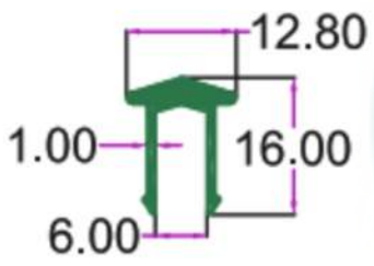
SEC.NO. 4890 WT. 0.555 TO 0.660 KG/12'
