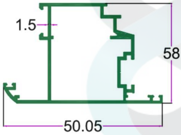
SEC.NO. 4775 WT. 3.320 TO 3.520 KG/I2'
