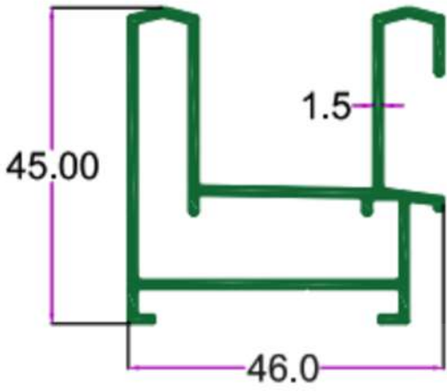
SEC. NO. 3313 WT. 3.270 TO 3.550 KG/12'
