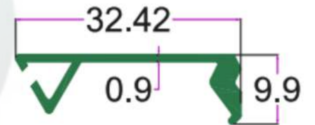
SEC. NO. 2055 WT. 0.900 TO 1.000 KG/15'
