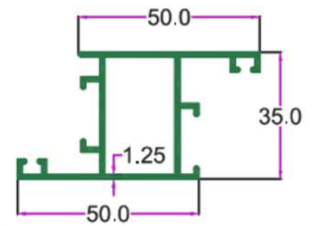
SEC. No. 3284 WT. 2.540 TO 2.800 KG/12'
