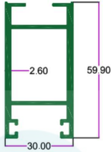
SEC. NO. 3991 WT. 3.900 TO 4.200 KG/12'
