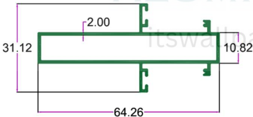
SEC. NO. 2201 WT. 3.900 TO 4.400 KG/15'
