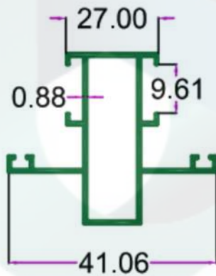
SEC. NO. 3521 WT. 3.000 TO 3.300 KG/12'
