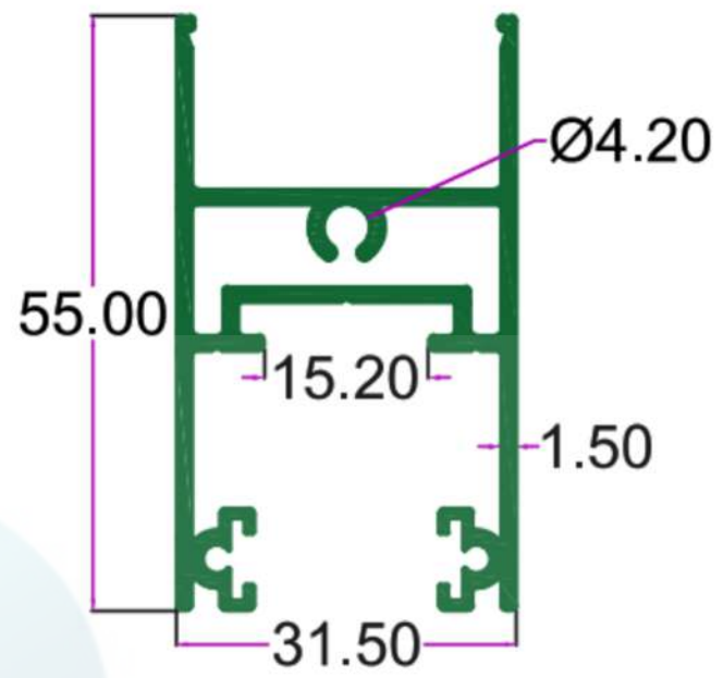
SEC.NO. 5240 WT. 3.315 TO 3.565 KG/I2'
