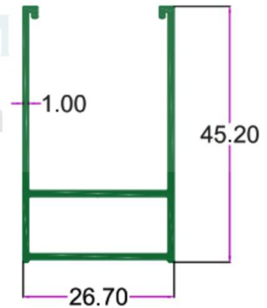
SEC.NO. 5215 WT. 1.430 TO 1.680 KG/12'
