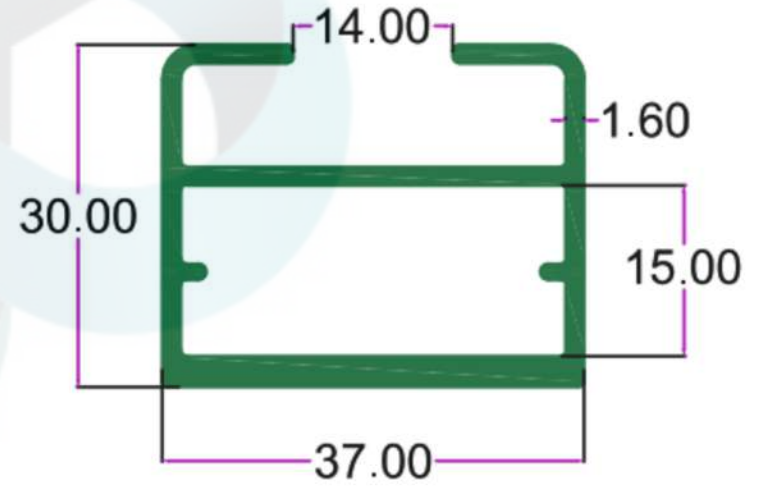
SEC. NO. 4874 WT. 2.720 TO 2.950 KG/12'
