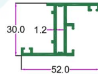
SEC. NO. 3525 WT. 1.650 TO 1.850 KG/12'
