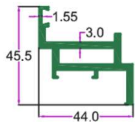
SEC. NO. 2118 WT. 3.900 TO 4.100 KG/12'
