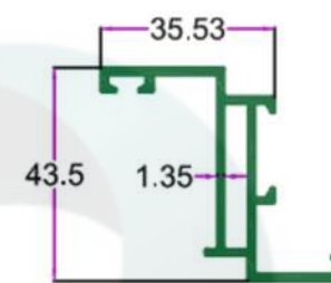
SEC. NO. 3262 WT. 2.070 TO 2.300 KG/12'
