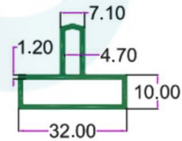
SEC.NO. 4277 WT. 1.440 TO 1.650 KG/12'
