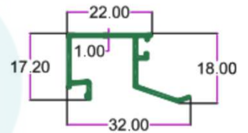
SEC. NO. 4767 WT. 0.760 TO 0.860 KG/12'
