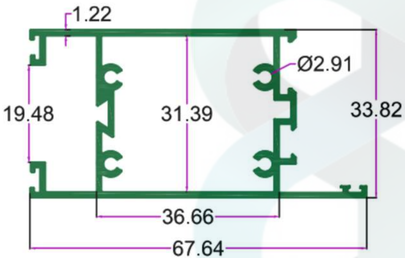
SEC. NO. 4769 WT. 6.550 TO 6.800 KG/12'
