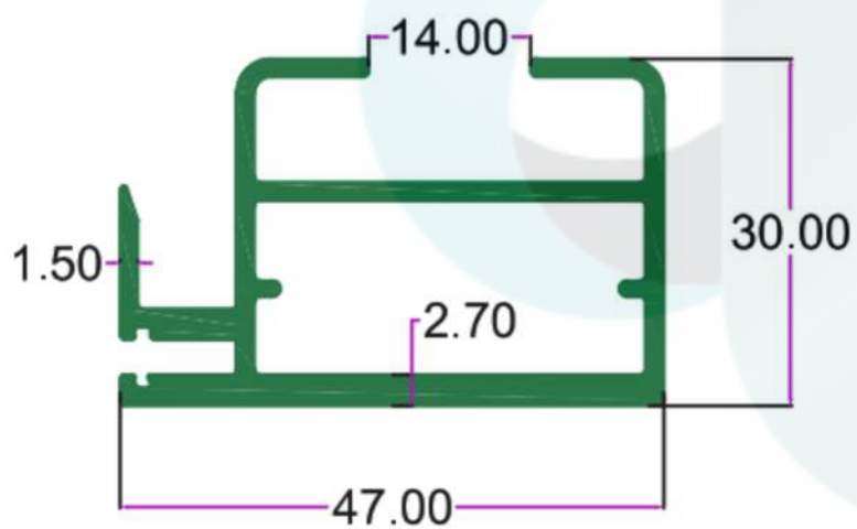
SEC.NO. 4977 WT. 3.375 TO 3.570 KG/12'
