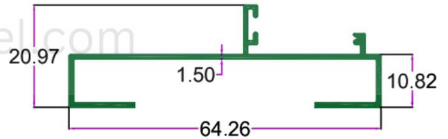
SEC. NO. 2202 WT. 2.600 TO 3.100 KG/15'
