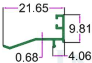
SEC. NO. 4773 WT. 0.600 TO 0.700 KG/12'
