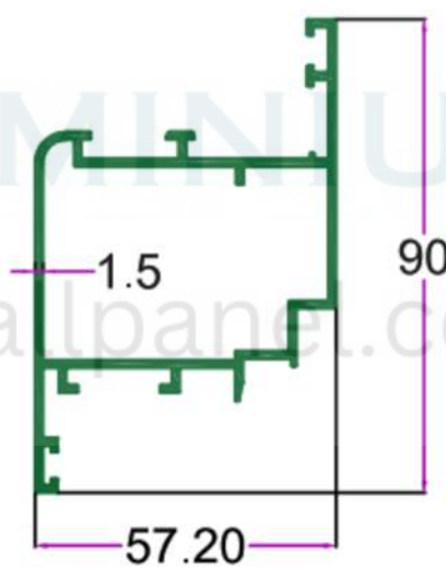
SEC. NO. 3940 WT. 4.400 TO 4.80 KG/12'
