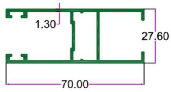
SEC.NO. 5120 WT. 2.810 TO 3.060 KG/12'
