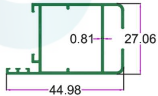
SEC. NO. 3464 WT. 3.500 TO 3.700 KG/12'
