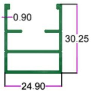
SEC.NO. 4992 WT. 1.110 TO 1.210 KG/12'
