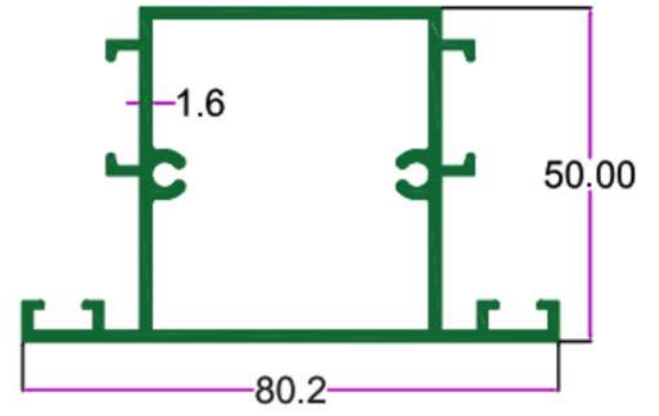
SEC. NO. 2213 WT. 6.800 TO 7.100 KG/15'
