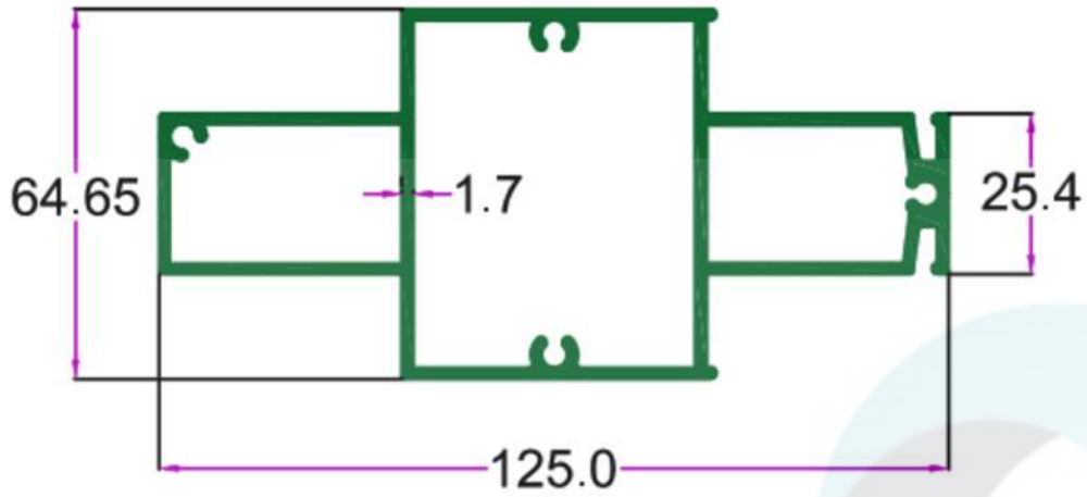
SEC. NO. 2062 WT. 7.800 TO 8.000 KG/12'
