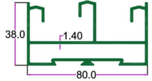
SEC. NO. 3314 WT. 4.30 TO 4.50 KG./ 12'
