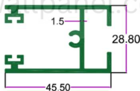
SEC. NO. 3651 WT. 2.500 TO 2.750 KG/12'
