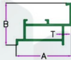
Z LINE SECTION
