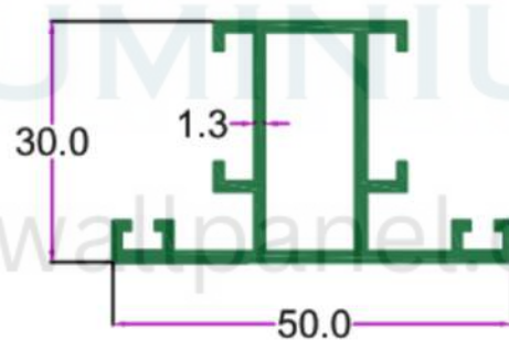
SEC. NO. 3524 WT. 1.900 TO 2.200 KG / 12'
