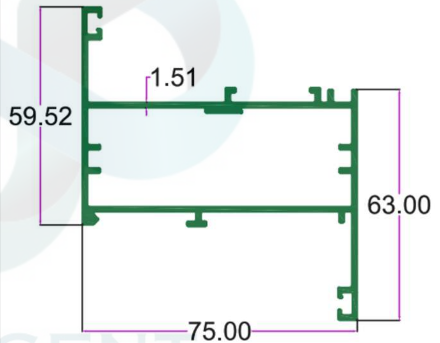
SEC.NO. 5115 WT. 5.030 TO 5.280 KG/12'
