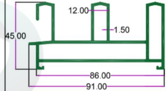
SEC. NO. 4272 WT. 5.750 TO 6.100 KG/12'
