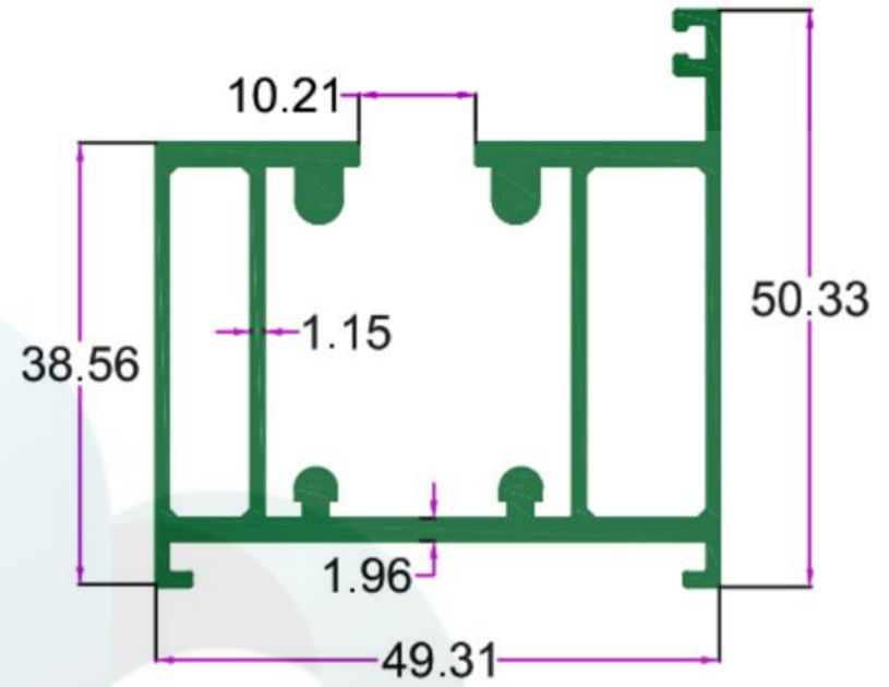
SEC. NO. 5008 WT. 8.860 TO 9.000 KG/12'
