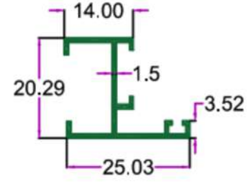
SEC. NO. 3522 WT. 1.550 TO 1.750 KG/12'
