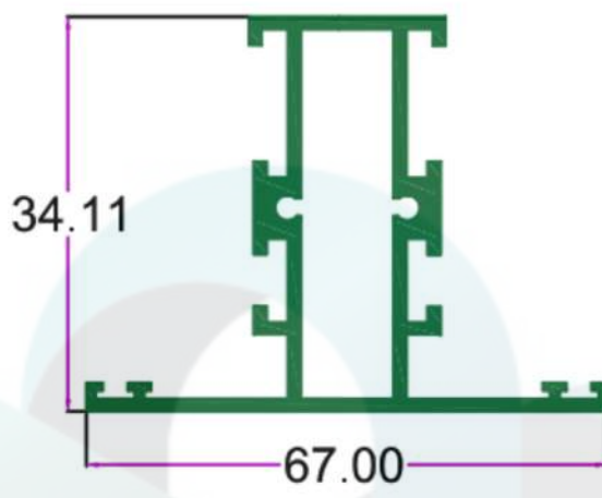
SEC. NO. 3779 WT. 4.50 TO 4.80 KG/12'
