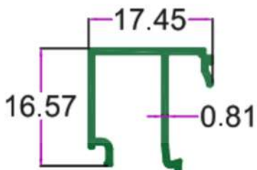
SEC. NO. 4770 WT. 1.030 TO 1.130 KG/12'
