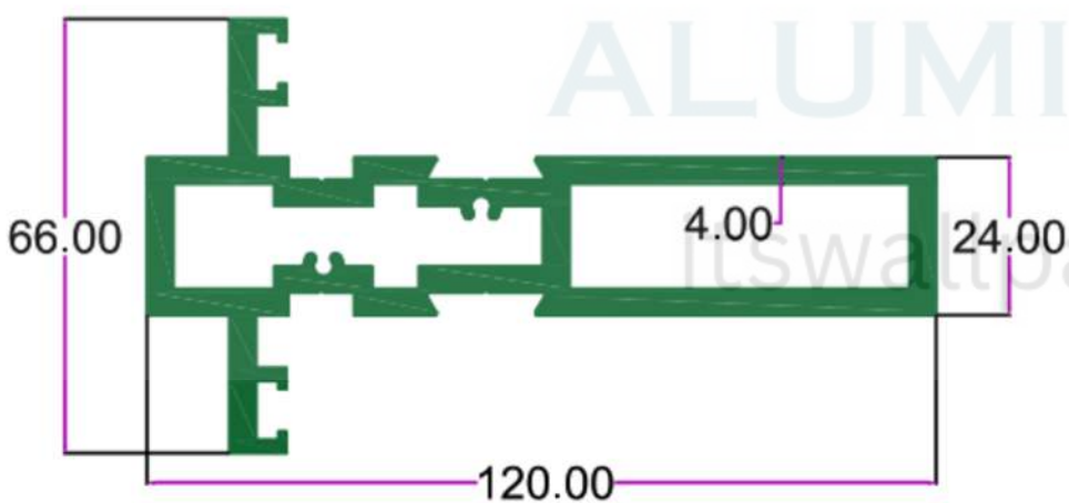
SEC. NO. 3611 WT. 13.300 TO 14.700 KG/12' SEC. NO. 3647(T 2MM) WT. 7.500 TO 8.250 KG/12'
