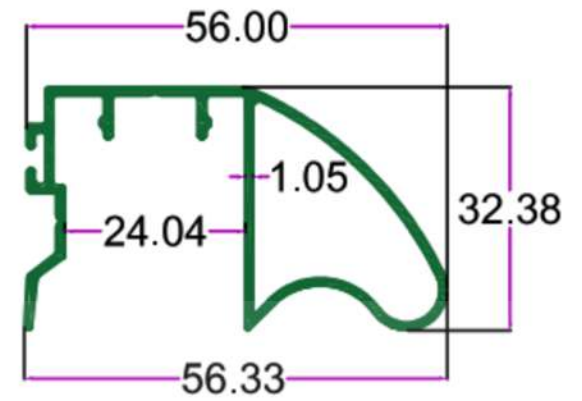
SEC.NO. 4847 WT. 2.580 TO 2.850 KG/12'
