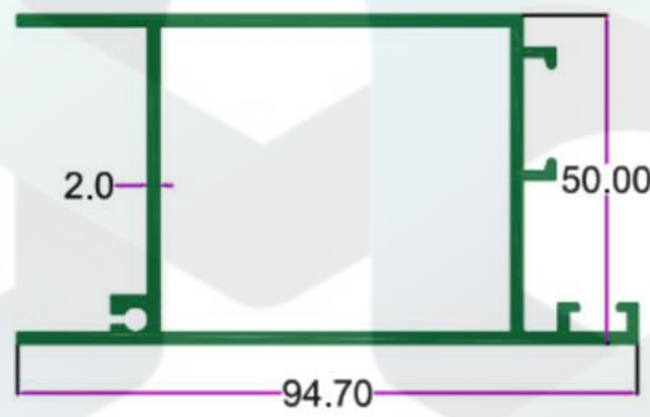
SEC. NO. 2214 WT. 7.250 TO 7.500 KG/15'
